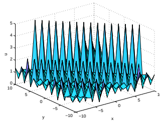
Fig. 2: The solution (19) for t = 0 , a = -\frac{1}{2}, b = \frac{1}{2}, n = 3, m = 8 , k_1 = l_1 = \lambda_1 = k = 1 , C_5 = C_6 = 1 .
