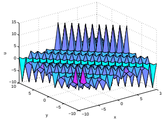
Fig. 5: The solution (25) for t = 0 , a = b = \frac{1}{2}, n = 3, m = 5 , k_1 = l_1 = \lambda_1 = k = 1 , C_{11} = C_{12} = 1 .
