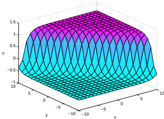
Fig. 4: The solution (24) for t = 0 , a = b = \frac{1}{2}, k_1 = l_1 = k = 1 , \lambda_1 = -1, n = 3, m = 5 , C_9 = 2, C_{10} = -1 .
