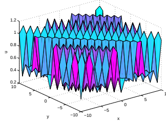
Fig. 8: The solution (28) for t = 0 , a = b = \frac{1}{2}, k_1 = l_1 = k = 1 , \lambda_1 = -1, n = 3, m = 2 , g = 0, C_{17} = C_{18} = 1 .
