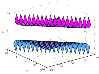
Fig. 11: The solution (14) for t = 0 , a = b = \frac{1}{2}, k_1 = l_1 = k = 1 , \lambda_1 = -2, n = 3, m = 4 , C_1 = 1, C_2 = 0 .
