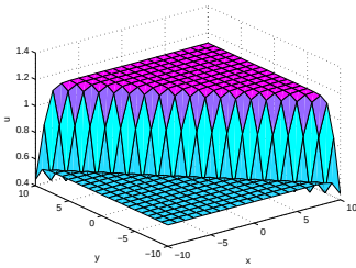
Fig. 1: The solution (18) for t = 0 , a = b = \frac{1}{2}, k_1 = l_1 = k = 1 , \lambda_1 = -1, n = 3, m = 8 , C_3 = 2, C_4 = -1 .
