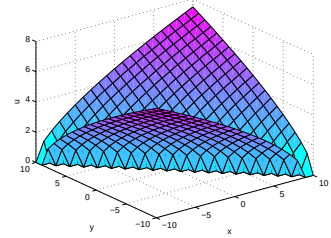
Fig. 9: The solution (29) for t = 0 , a = 1, b = \frac{1}{2}, k_1 = l_1 = k = 1 , \lambda_1 = -1, n = 3, m = 2 , g = 1, C_{19} = 1, C_{20} = 0 .
