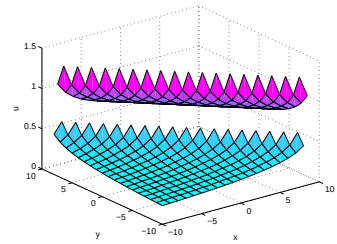
Fig. 3: The solution (20) for t = 0 , a = b = \frac{1}{2}, k_1 = l_1 = k = 1 , \lambda_1 = -2, n = 3, m = 8 , C_7 = 1, C_8 = 0 .
