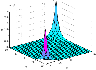
Fig. 7: The solution (27) for t = 0 , a = b = \frac{1}{2}, n = 3, m = 2 , k_1 = l_1 = \lambda_1 = k = 1 , g = 0, C_{15} = C_{16} = 1 .
