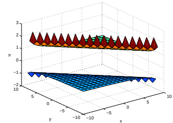
Fig. 6: The solution (26) for t = 0 , a = b = \frac{1}{2}, k_1 = l_1 = k = 1 , \lambda_1 = -2, n = 3, m = 5 , C_{13} = 1, C_{14} = 0 .
