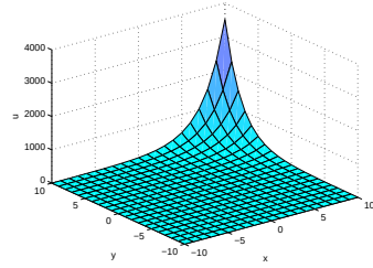
Fig. 13: The solution (67) for t = 0 , a = b = \frac{1}{2}, n = 6, m = 2 , k_1 = l_1 = \lambda_1 = k = 1 , C_{26} = 1 .
