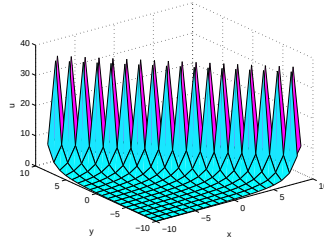
Fig. 12: The solution (36) for t = 0 , a = b = \frac{1}{2}, k_1 = l_1 = k = 1 , \lambda_1 = -2, n = m = 3 , C_{21} = 1, C_{22} = 0 .
