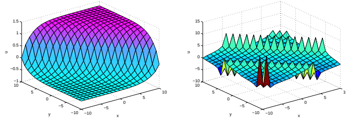
Fig. 10: The solution u(x, y, t) for t = 0, a = b = \frac{1}{2}, k_1 = l_1 = k = 1, \lambda_1 = -1, n = 3, m = 5, C_{23} = C_{24} = 0 .
