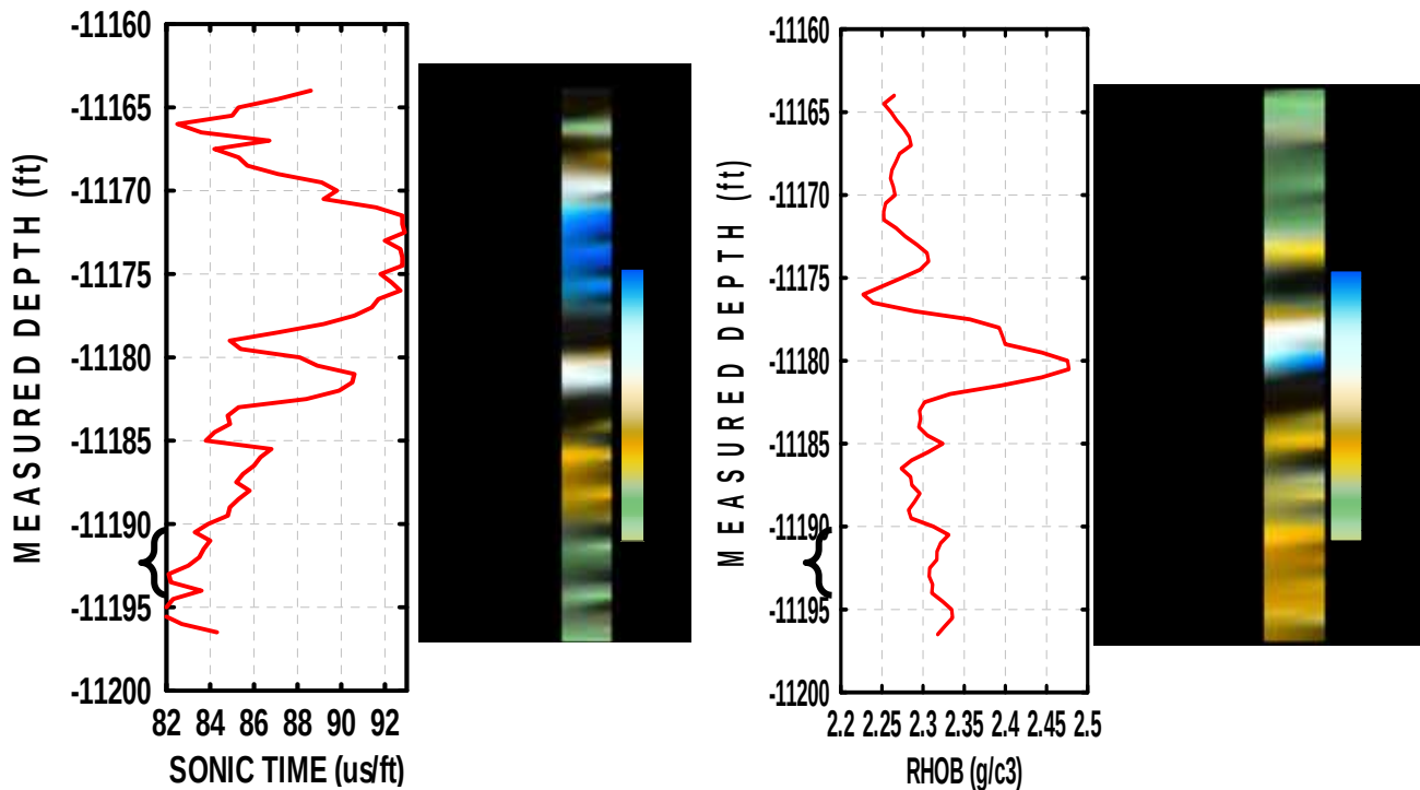
Figure 6: Logs of Sonic Time and Density (RHOB) Within the Depth Interval of Reservoir for Well 4. Right to each Plot is a Respective Surface Maps Generated to Show Comparison within the Interval, also the Legend Shows the Distribution of the Quantities with depth.
