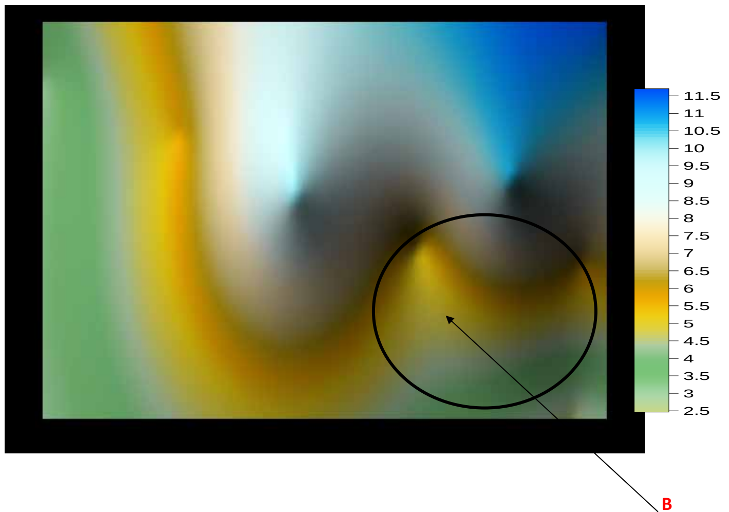
Fig 15: Coherence Amplitude in Time domain
