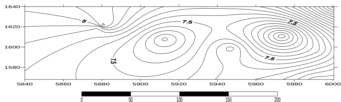
Figure 12: Amplitude time maps with contour maps at the base of delineated reservoir (2.769)
