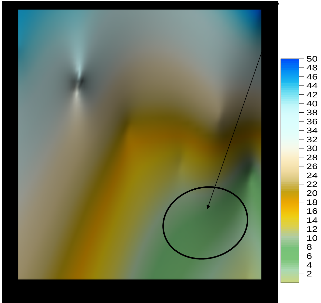
Fig 17: Coherence in Frequency
