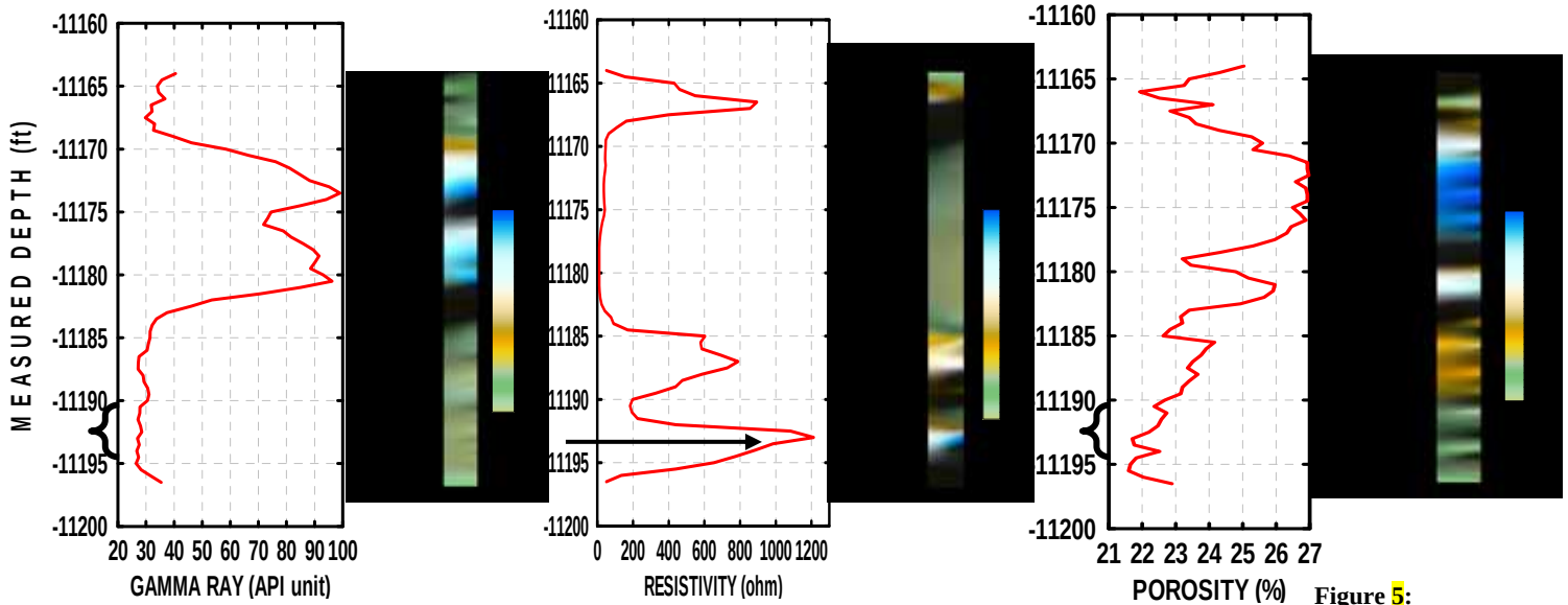
Figure 5: Logs of Gamma ray (GR), Resistivity (LLD) and Porosity within the Depth Interval of the Reservoir for Well 4. Right to each Plot is a Respective Surface Map Generated to Show Comparison within the Interval, also the Legend shows the Distribution of the Quantities with Depth
