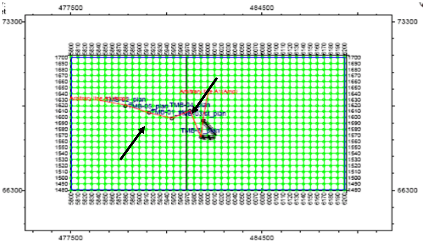
Figure 2. Base Map of 3-D Seismic Showing all Wells (well 4 and 5 are shown as TMB 04 and 05 with Arrows An Arbitrary Red Line Drawn to Connect the Six Wells in Field (courtesy: Chevron Nig Ltd).
