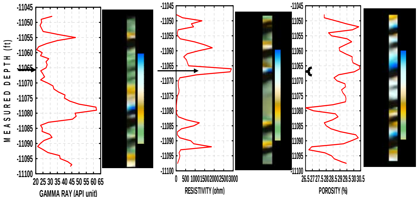
Figure 7: Logs of Gamma ray (GR), Resistivity (LLD) and Porosity within the Depth Interval of Reservoir for Well 5. Right to each Plot is a Respective Surface Maps Generated to Show Comparison Within the Interval, also the Legend shows the Distribution of the Quantities with Depth.
