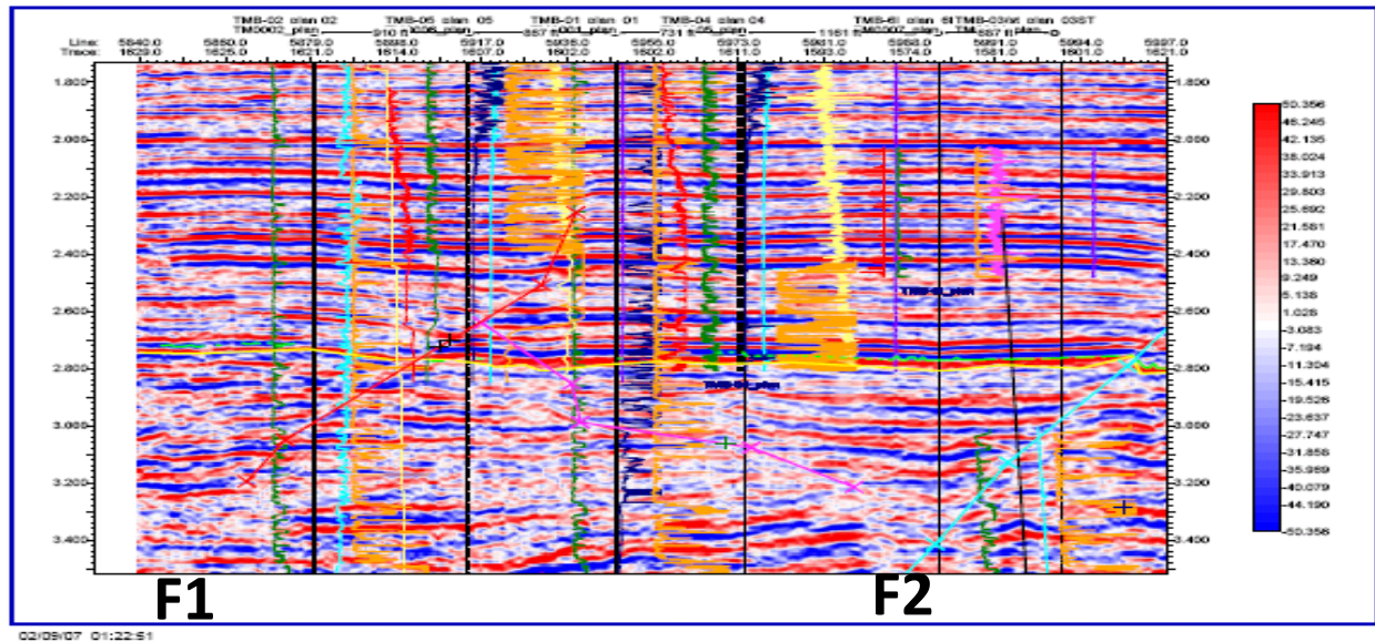
Figure9: Seismic Section Showing an Arbitrary Line Indicating Two Major Faults, F1 and F2 Bounding the Wells at the Reservoir Interval under analysis (2.752-2.768 sec). The well Locations are indicated above the seismic section.
