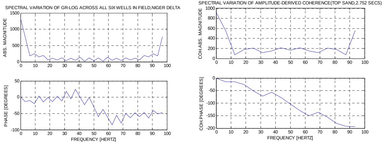
Fig 10: lines plots of amplitude derived coherence and gamma log
