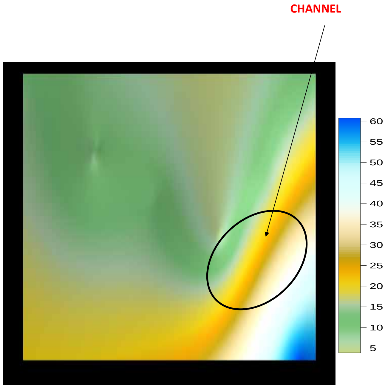
fig 16: Coherence in Phase
