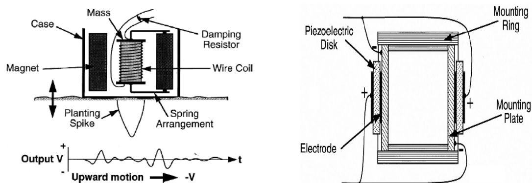
Figure 1.1: Schematic Representation of: (i) Geophone and (ii) Hydrophone (Modified from [3])
