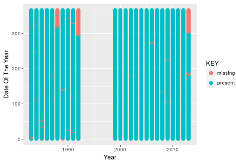
Figure 2.11: Missing values of SIS
