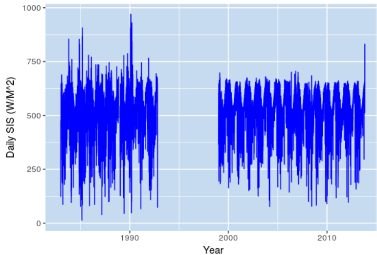
Figure 4.8: Time series plot of the SIS
