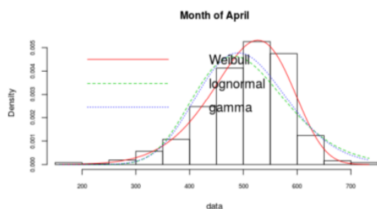
Figure 4.1: fitted distribution for April
