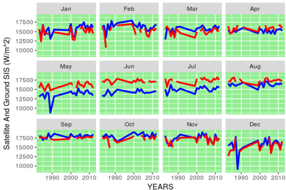
Figure 4.11: SIS variation by month. Combined line graphs of ground and satellite data. The red lines represents the data collected from the ground while the blue lines represent the satellite data.
