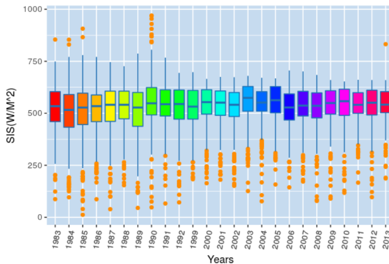
Figure 4.7: SIS radiation by Years
