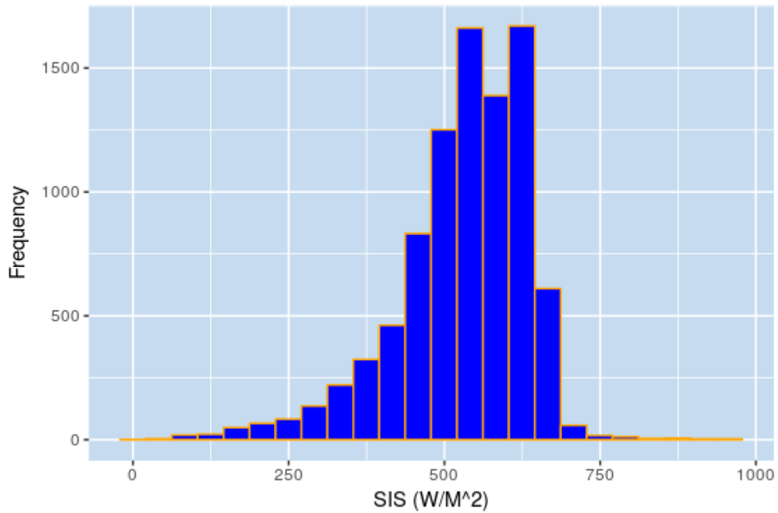
Figure 4.10: Histogram of SIS
