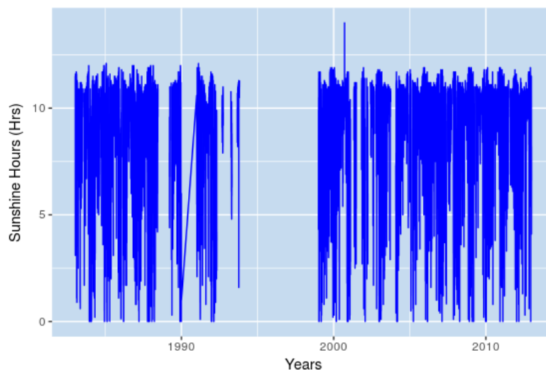
Figure 4.4: Daily variation of sunshine hours over the years
