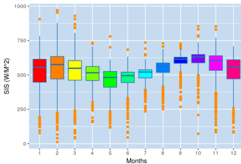
Figure 4.9: SIS radiation by months
