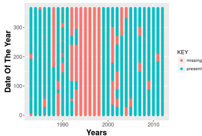
Figure 2.5: Missing values of sunshine hours.
