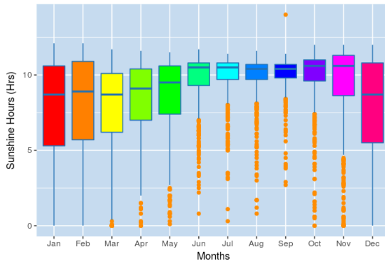
Figure 4.5: Sunshine hours by months
