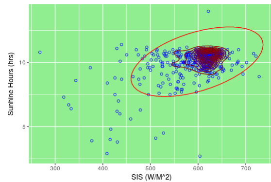
Figure 4.13: Scatter plot in September
