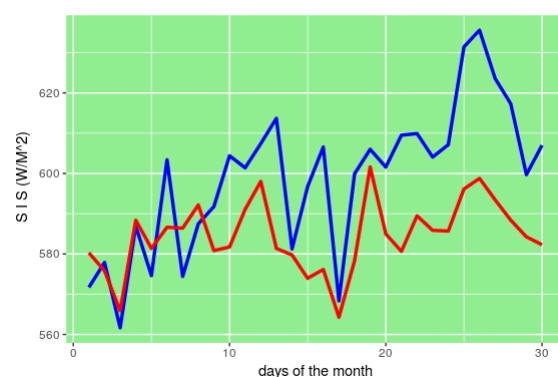
Figure 4.15: Variation of SIS over September
