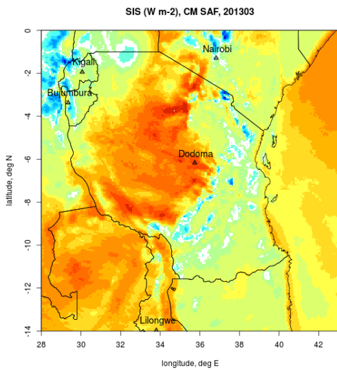
Figure 2.1: SIS plot for satellite data
