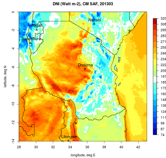
Figure 2.2: Average DNI over Tanzania in 2013
