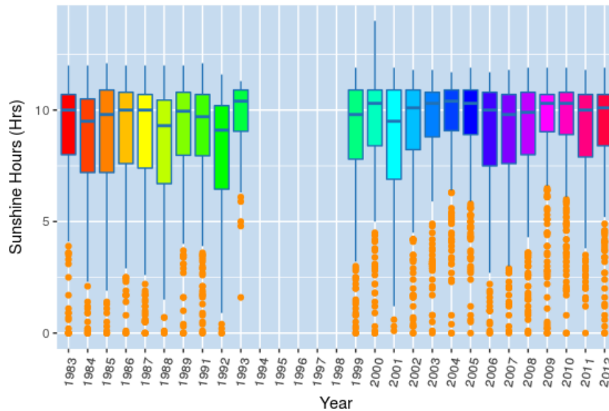
Figure 4.3: Sunshine hours by years
