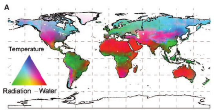
Figure 1.1: Geographic distribution of potential climatic constraints, temperature, radiation and water, to plant growth derived from long-term climate statistics. (Nemani et al., 2003)
