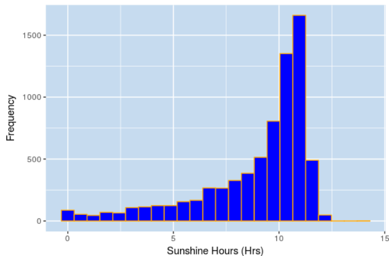
Figure 4.6: Histogram of sunshine hours
