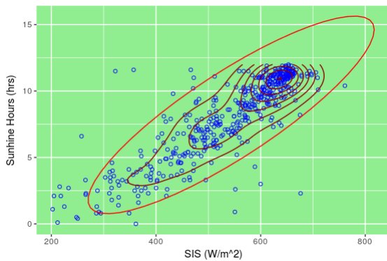
Figure 4.12: Scatter plot in February
