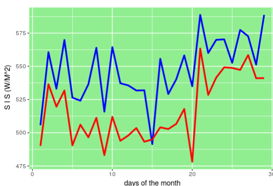
Figure 4.14: Variation of SIS over February
