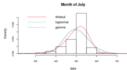
Figure 4.2: fitted distribution for July
