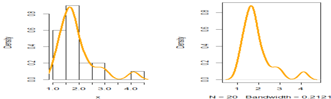
Figure 7: A Histogram and density plot for the Relief times of 20 patients (Data set III)
