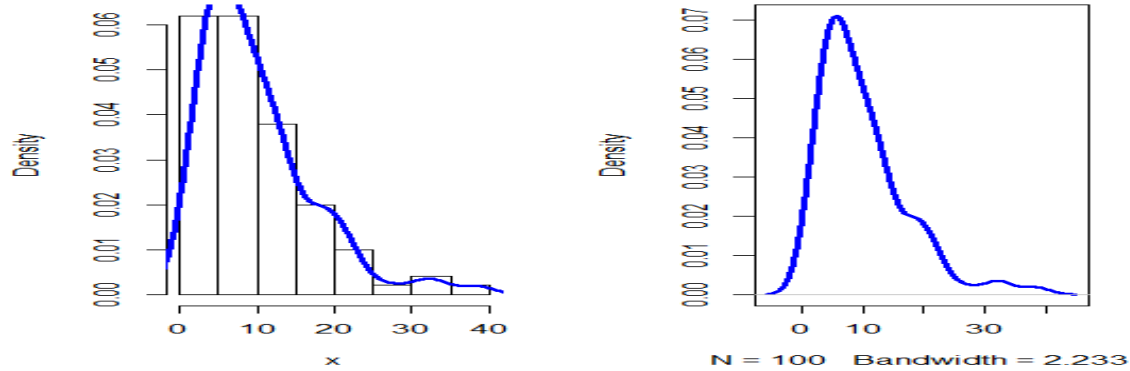
Figure 5: A histogram and density plot for the waiting times of bank customers (Dataset I)
