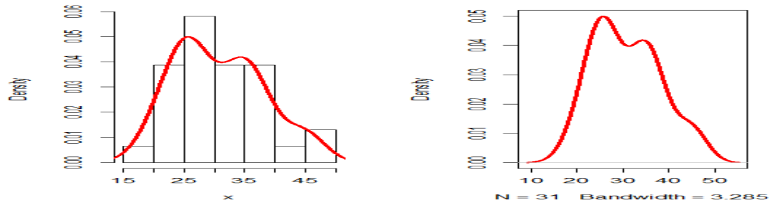
Figure 6: A Histogram and density plot for the strength of glass of windows (Data set II)
