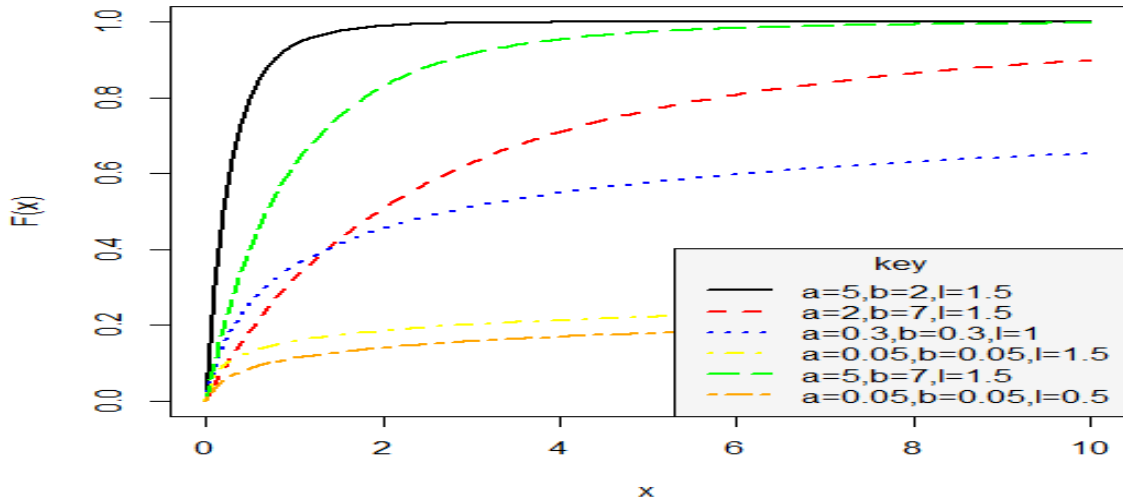
Figure 2: Graph of CDF of the LED for different parameter values From the above cdf plot, the cdf increases when X increases, and approaches 1 when X becomes large, as expected.
