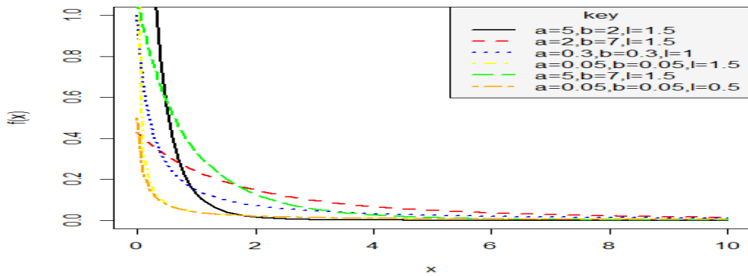
Figure 1: Graph of PDF of the LED for different parameter values Figure 1 indicates that the LED is a skewed distribution and such skewed to the right. This means that distribution can be very useful for datasets that are positively skewed.
