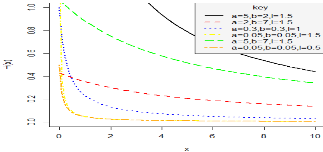
Figure 4: Plot of the hazard function of the LED for different parameter values
