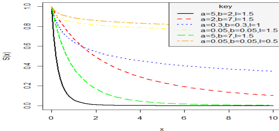
Figure 3: Plot of the survival function of the LED for different parameter values
