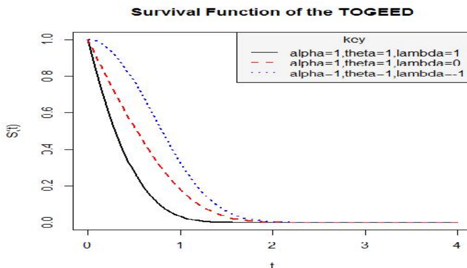
Figure 3.4.1: Survival function of the TOGEED at different parameter values.
