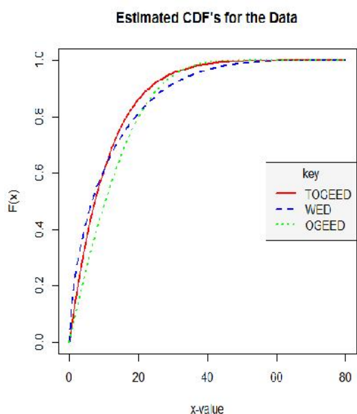
246 Figure 5.1: Histogram and estimated densities and CDF's of the TOGEED , OGEED and 247 WED for the bladder cancer dataset.
