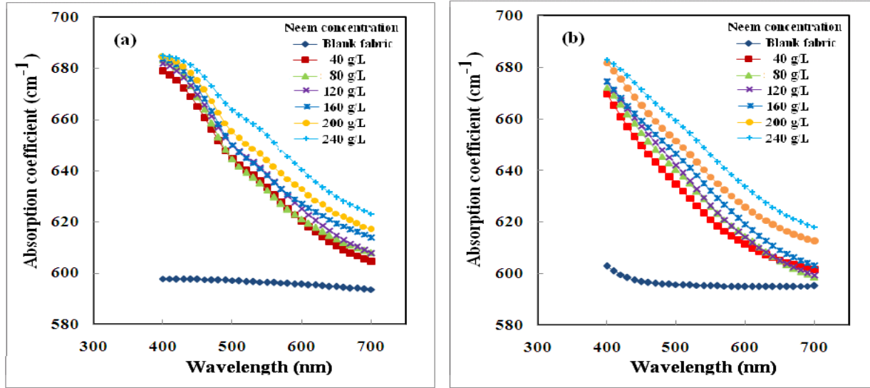
Fig. 4. Plots of the absorption coefficient values of undyed as well as neem dyed silk fabrics with different dye bath concentrations before (a) and after (b) exposure to artificial day light for 160 h against wavelength
