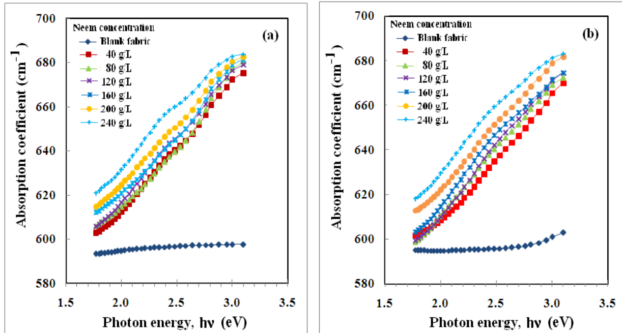
Fig. 5. Plots of the absorption coefficient values of undyed as well as neem silk fabrics with different dye bath concentrations before (a) and after (b) exposure to artificial day light for 160 h against photon energy ( h\nu )
