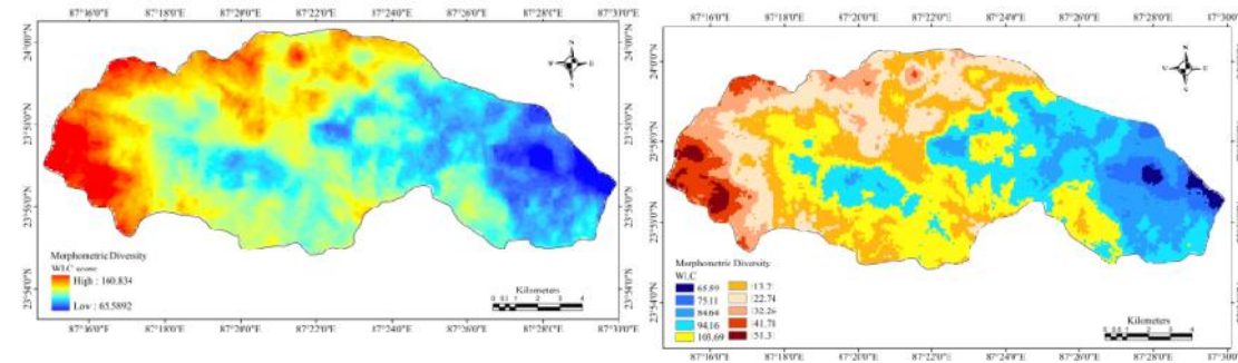
Fig 6 (a) Weighted Morphometric Diversity (b) Weighted classified Morphometric Diversity
