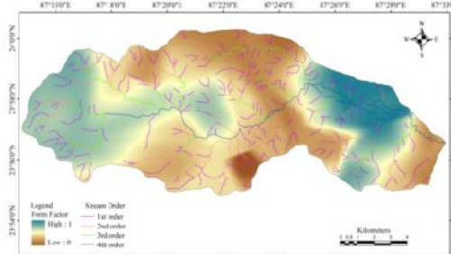
(R) Form Factor
