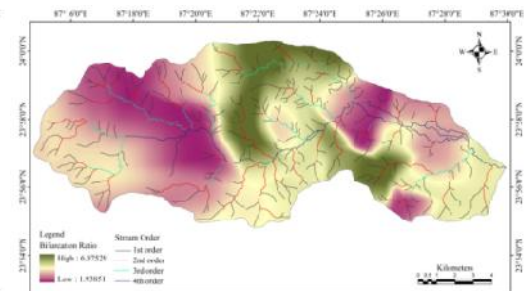
(J) Bifurcation Ratio
