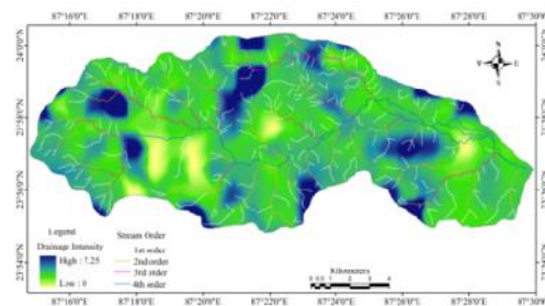
(S) Drainage Intensity
