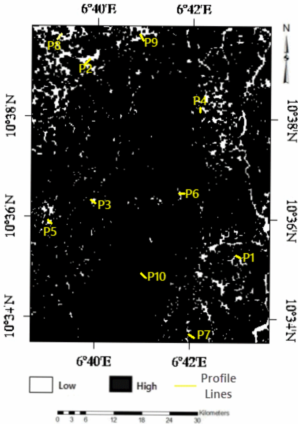
Figure 5: Low threshold zones within the study area
