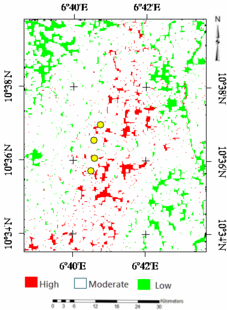
Figure 6: Relationship between gold mineralisation and alterations within the study area
