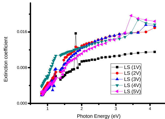
157 158 Figure 6: plot of extinction coefficient as a function photon energy
