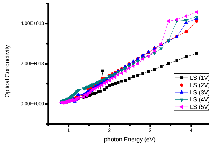
152 153 Figure 5: plot of optical conductivity as a function photon energy
