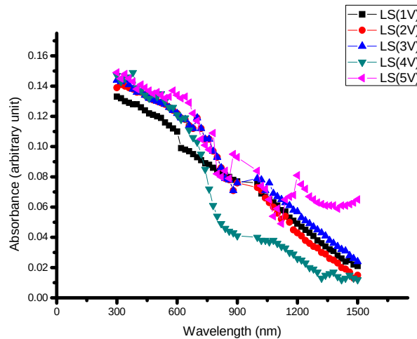
108 Figure 1: plot of absorbance as a function wavelength
