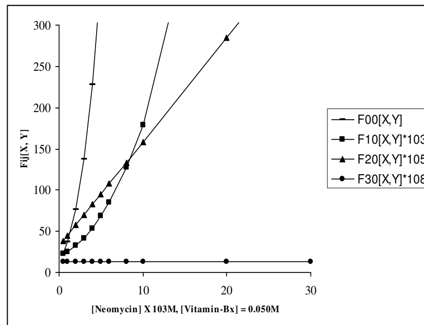
Fig. -1: Polarographic Characteristics and F_{ij}[X, Y] Values of [Zn- Neomycin – Vitamin-B x ] System
