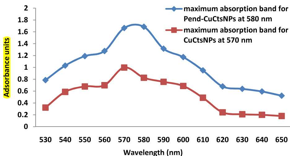
Figure 1: UV-Visible Spectral of CuCtsNPs and Pend-CuCtsNPs
