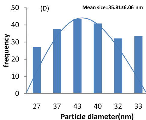
Figure 4. TEM Images of the Synthesized CuCtsNPs and Pend-CuCtsNPs (A and C) and their Particle Size Distribution Histograms ( B and D)
