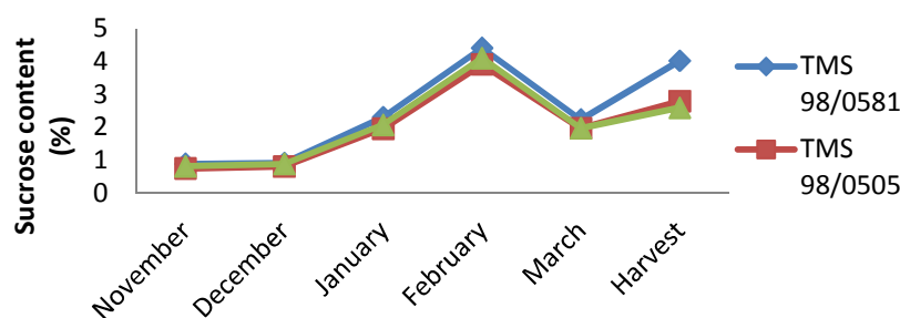
Fig. 1. Variation of sucrose content with month of maturity
