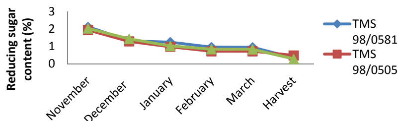
Fig. 2. Variation of reducing sugar content with month of maturity
