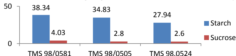
Fig.3. Composition of starch and sucrose content
