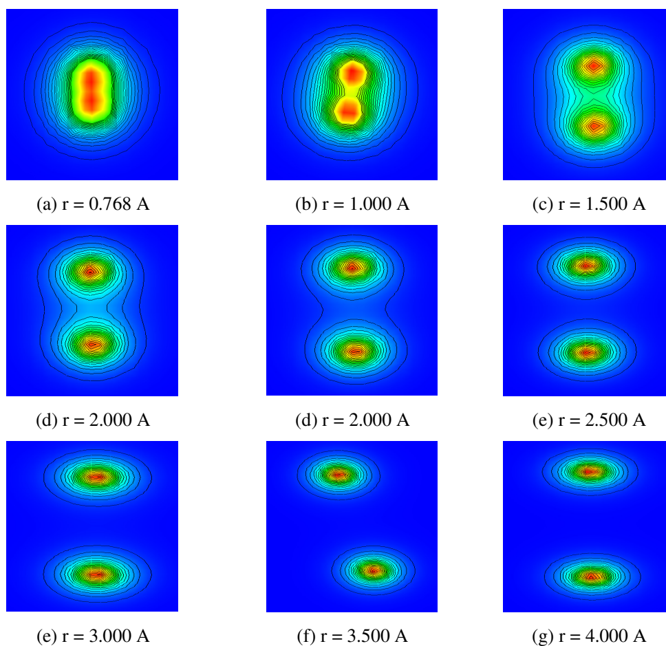
Figure 1.2: Contour plot of hydrogen dissociation from H_2 into 2H
