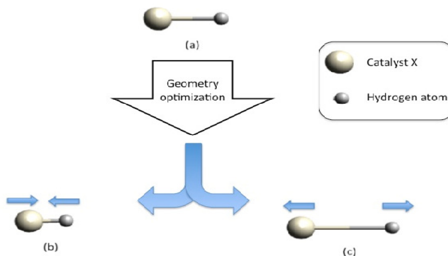
Figure 2.1: The original configuration of structure (a) will be optimized and transformed into structure (b) or structure (c). Structure (b) shows bigger relative bond strength value compared to structure (c).
