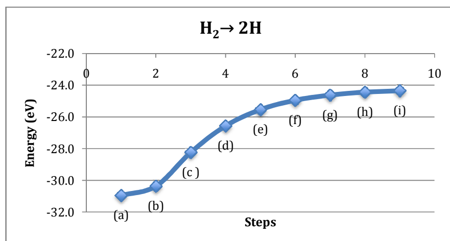
Figure 1.1: Total energy required for hydrogen dissociation ( H_2 to 2H ).
