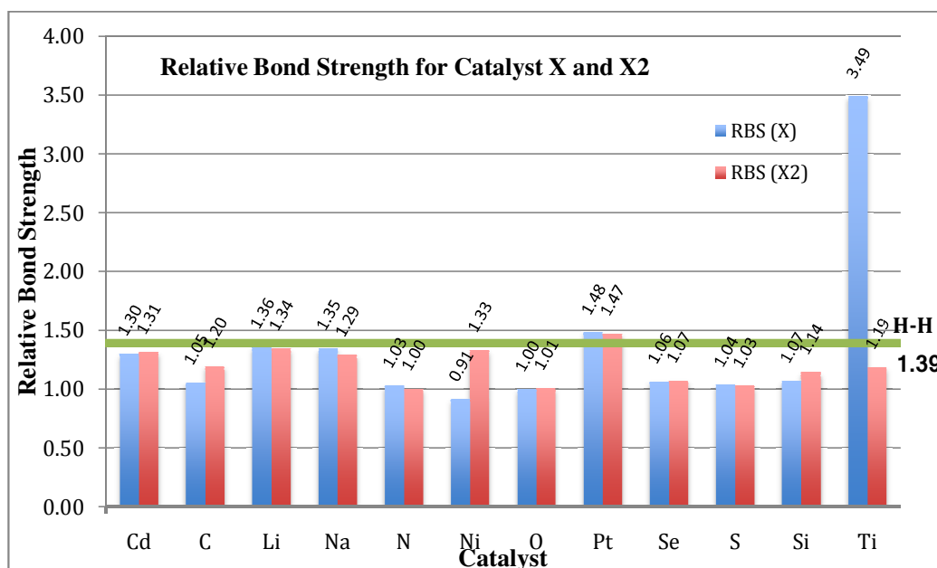
Figure 3.1: Relative bond strength for single atom (blue) and double atom (red)
