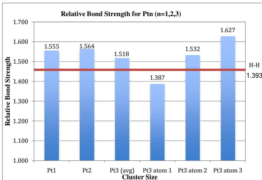
Figure 3.3: A graph of relative bond strength values for different configurations of Pt-H molecule.
