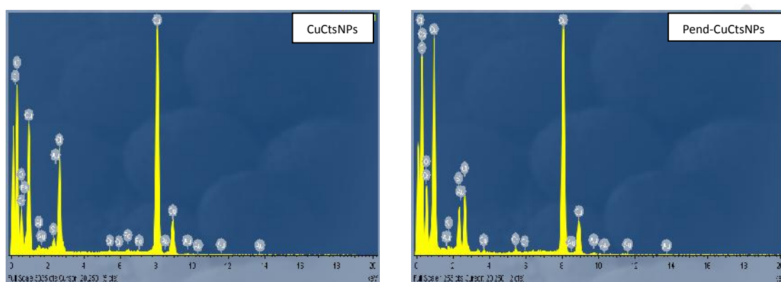
Figure 5: EDX Spectra of the Synthesized CuCtsNPs and Pend-CuCtsNPs
