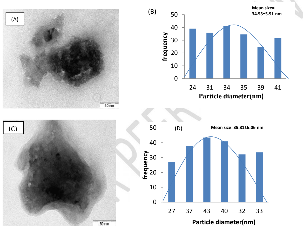
Figure 4. TEM Images of the Synthesized CuCtsNPs and Pend-CuCtsNPs (A and C) and their Particle Size Distribution Histograms ( B and D)
