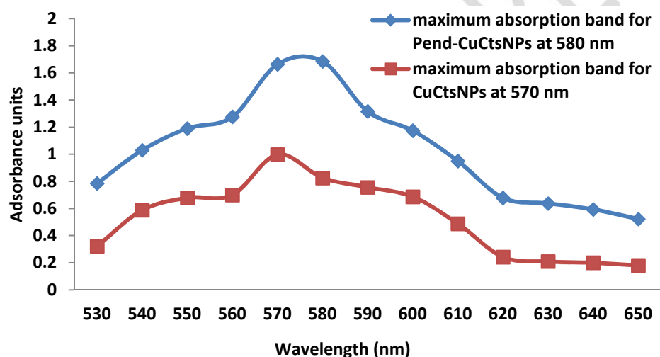
Figure 1: UV-Visible Spectral of CuCtsNPs and Pend-CuCtsNPs
