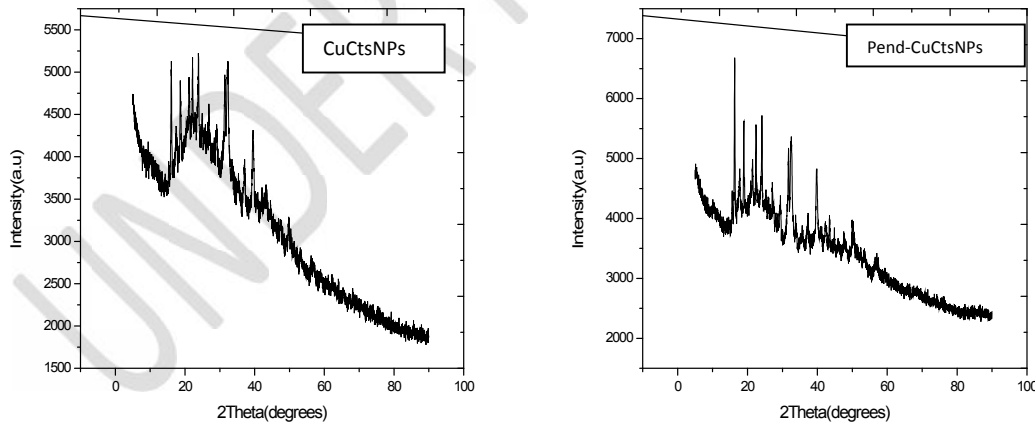
Figure 3: PXRD Diffractogram of CuCtsNPs and Pend-CuCtsNPs
