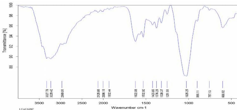
Figure 2: FT-IR spectrum for Pend-CuCtsNPs
