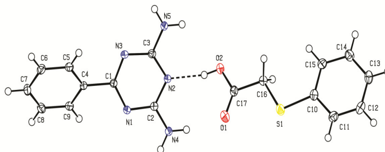
Fig. 2 ORTEP view of DAPT:PTAA with displacement ellipsoids drawn at 50% probability level
