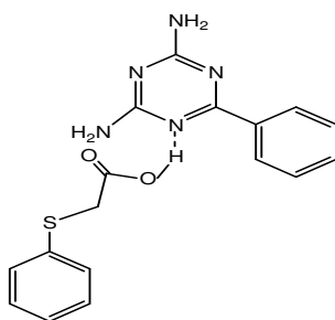
Fig. 1. The chemical structure of DAPT:PTAA
