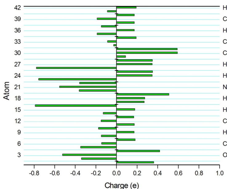
Fig.7 Mulliken charge of DAPT:PTAA
