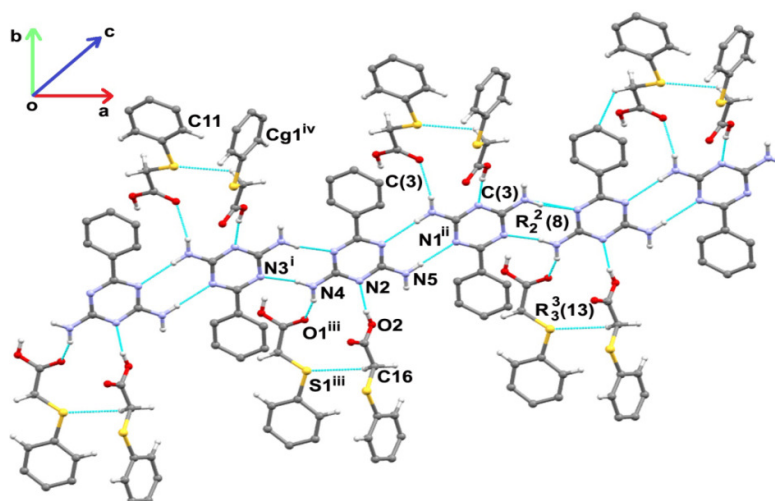
Fig. 3 Supramolecular sheets through N-H...N, N-H...O, C-H...S hydrogen bonds and C-H... \pi interaction. [Symmetry codes: (i) -1/2+x, 1-y, z ; (ii) 1/2+x, 1-y, z ; (iii) 1/2-x, y, -1/2+z ; (iv) 1/2-x, y, 1/2+z ].
