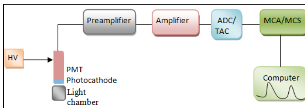
Figure 1. Block diagram of a typical Fluorescence Spectroscopy
