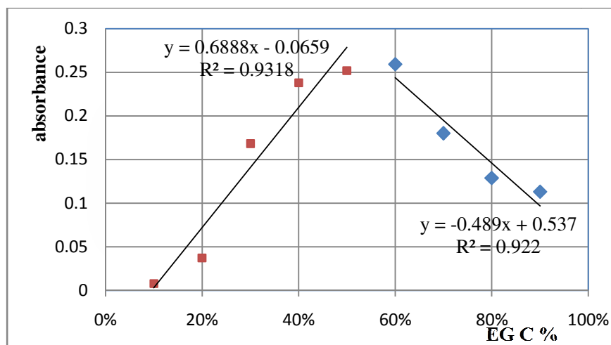
Figure 5. Calibration graph for the determination of ethylene glycol (C %)
