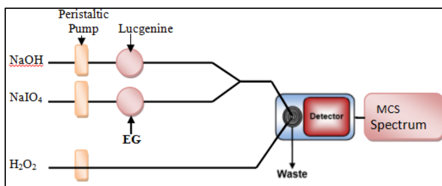
Figure 3. The flow injection analysis used for CL determination of EG
