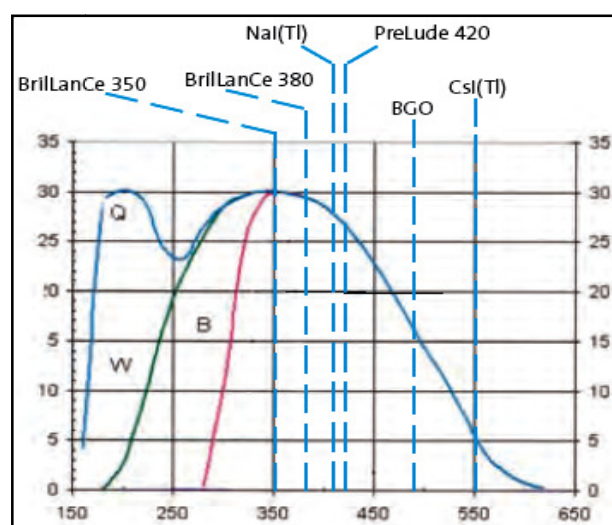
Figure 2. Maximum emission points of various scintillators compared to quantum efficiency of a bialkali ETI9266 PMT with (B) Borosilicate, (W) UV glass and (Q) Quartz face plates (Q.E. data courtesy of Electron Tubes, Inc.)
