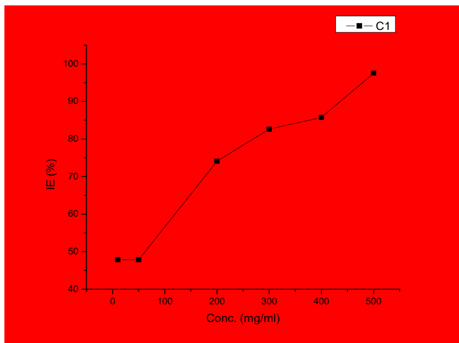
Fig 4: Inhibition efficiency against concentration of Costus afar
