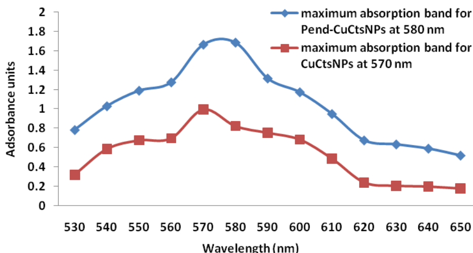
Fig. 1. UV-Visible Spectral of CuCtsNPs and Pend-CuCtsNPs
