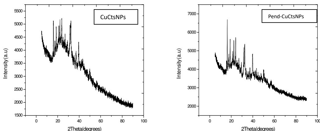
Fig. 3. PXRD Diffractogram of CuCtsNPs and Pend-CuCtsNPs
