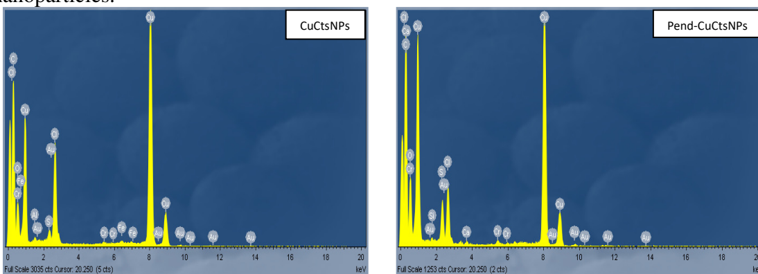
Fig. 5. EDX Spectra of the Synthesized CuCtsNPs and Pend-CuCtsNPs
