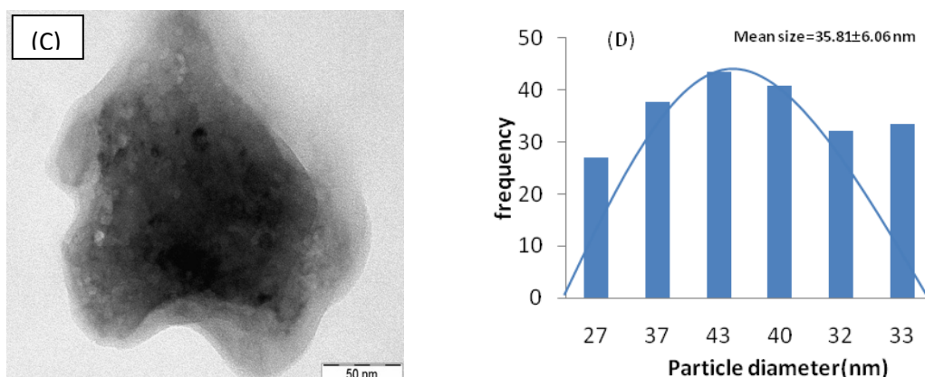
Fig. 4. TEM Images of the Synthesized CuCtsNPs and Pend-CuCtsNPs (A and C) and their Particle Size Distribution Histograms ( B and D)
