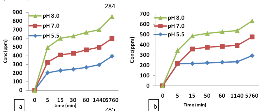
Fig. 6. Concentration of pendimethalin released from (a) 0.8% and (b) 0.3% loaded CuCtsNPs
