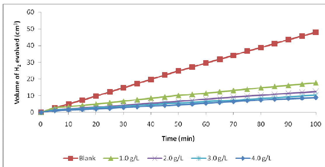
112 Fig. 2. Variation of volume of H 2 gas evolved (cm 3 ) with time (min) for mild steel corrosion in 1 113 M H 2 SO 4 in the absence and presence of Eremomastax polysperma leaf extract at 30 °C
