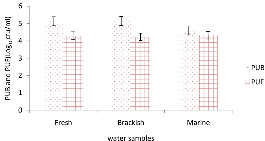
Fig.1: Variations in petroleum utilizing bacteria and petroleum utilizing fungi in tri-aquatic environment
