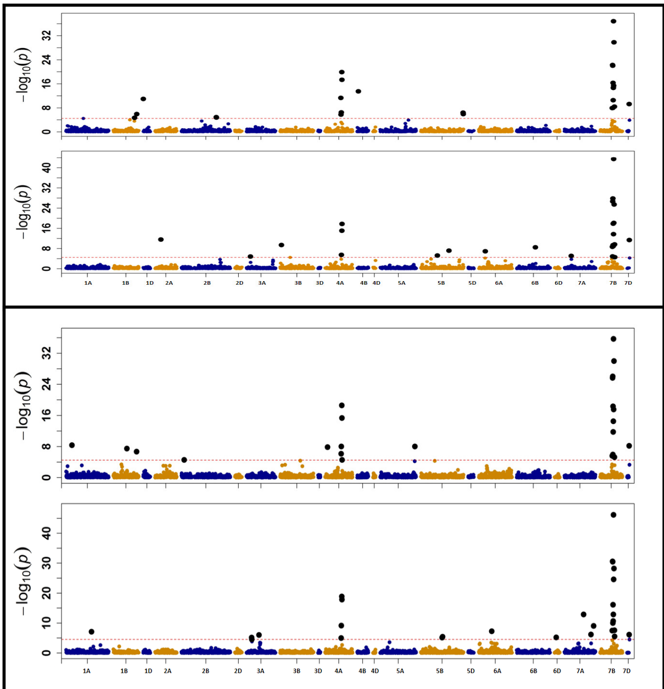
Figure (7): Manhattan plot for stem rust results obtained from genome-wide association mapping across years and locations.
