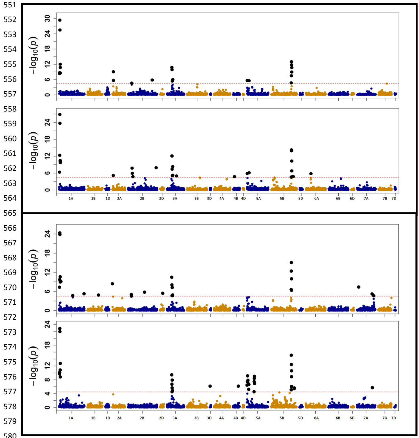
Figure (8): Manhattan plot for leaf rust results obtained from genome-wide association mapping across years and locations.
