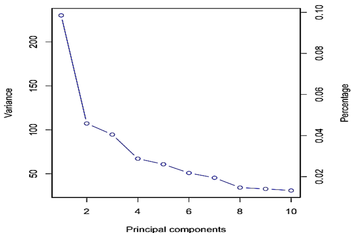
Figure (4): The percentage of variance explained by principal component ( PCA)
