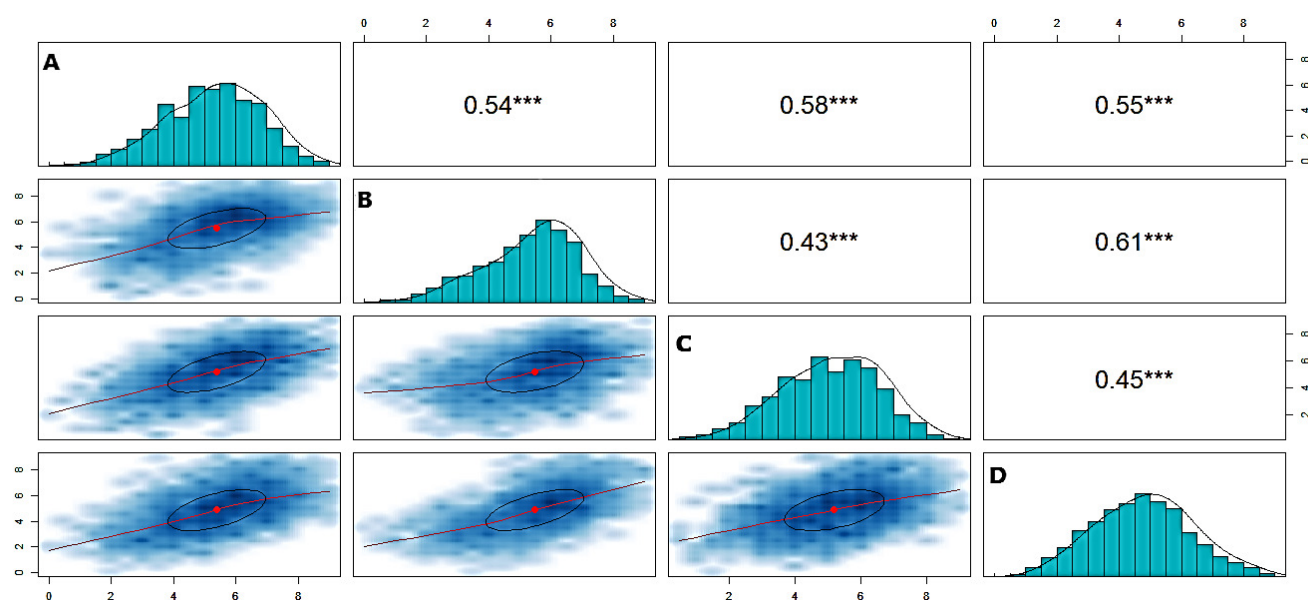
278 Figure 2: Histogram, scatterplot and correlation matrix for the average coefficient of infection 279 (ACI) for stem rust among 2016 locations; Elkhazan (A), and Elbostan(C); and 2017 280 Locations; Elbostan (D) and Elkhazan (B).
