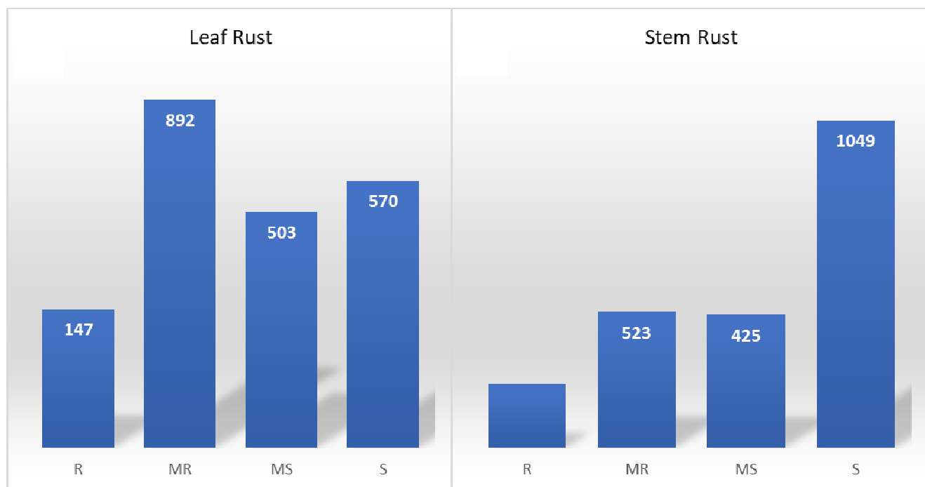
Figure3: Distribution of the overall all performance of the tested wheat accessions to the four classes of infection types i.e. resistant (R), moderately resistance (MR), moderately susceptible (MS) and Susceptible (S) to leaf and stem rust under the field conditions across locations and seasons.
