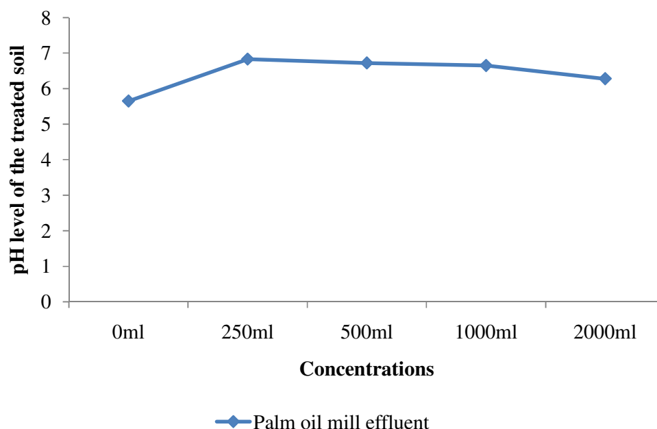
Figure 1: Effect of concentrations of palm oil mill effluent on the soil pH
