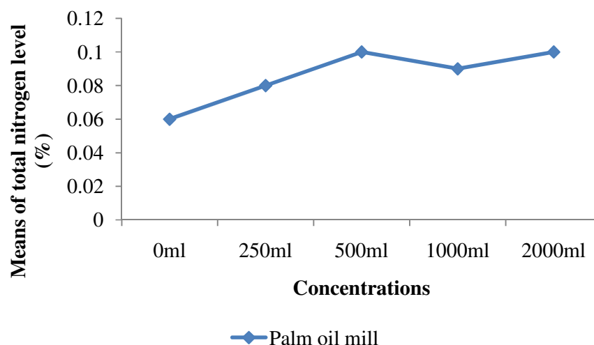
Figure 3: Effect of concentrations of palm oil mill effluent on total nitrogen content of the polluted soil
