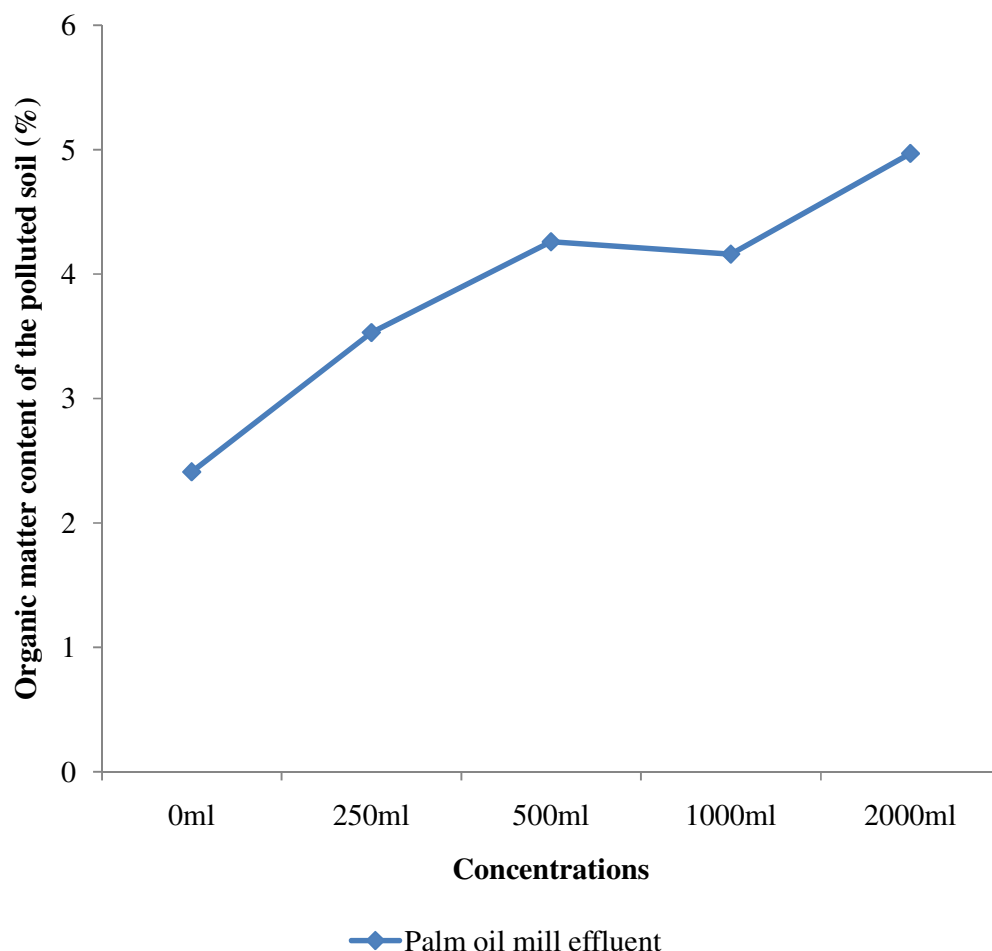
Figure 2: Effect of concentrations of palm oil mill effluents on soil organic matter
