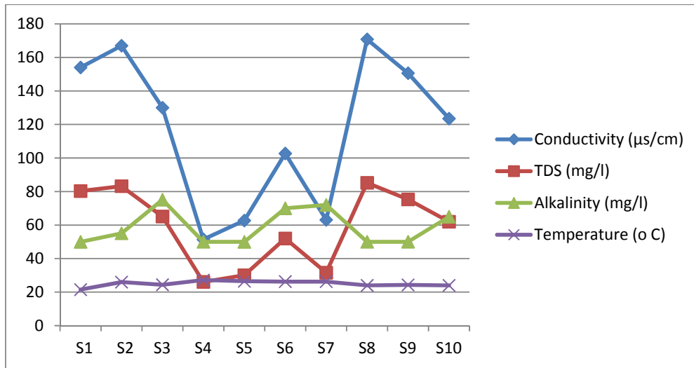
444 Fig. 3 : Cond, TDS , Alkalinity and Temp. of Waters from Study Area
