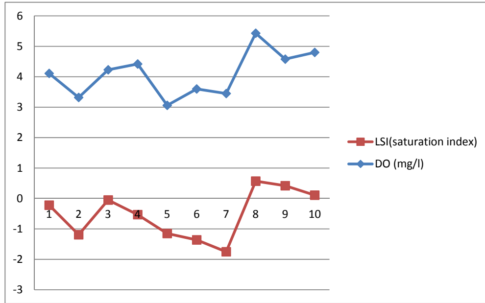
438 Fig. 2 : DO , LSI from Study Area
