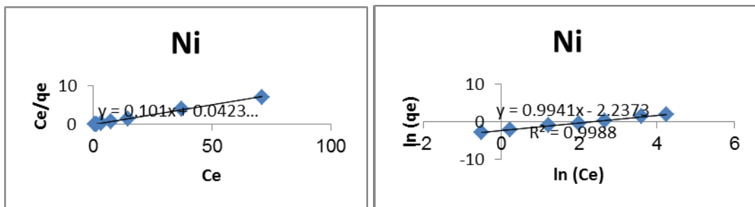
307 Figure 7. Adsorption isotherms of Cd +2 , Fe +3 , and Ni +2 based on the Langmuir and 308 Freundlich models
