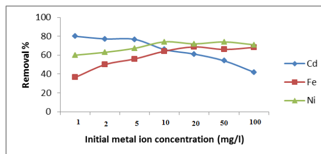
Figure 4. Initial heavy metal ion concentration (mg/l) affecting on the removal of \text{Cd}^{+2} , \text{Fe}^{+3} and \text{Ni}^{+2} from the solution (size < 0.5 mm; m = 0.5\text{g} ; V = 50\text{ml} pH = 6; t = 180 min)
