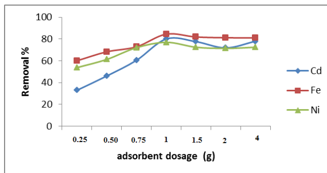
253 Figure 5. Adsorbent dose affecting on the removal of \text{Cd}^{+2} , \text{Fe}^{+3} and \text{Ni}^{+2} , from the 254 solution ( C_i = 2 ppm; size < 0.5 mm; pH= 6; V=50ml; t=180 min)
