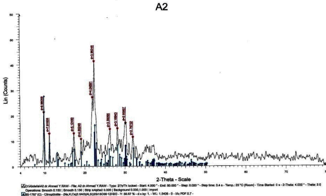
Figure 1. The XRD pattern of the sample confirming its Clinoptilolite mineralogy.
