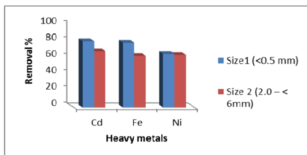
Figure 2. Adsorbent particle size affecting on the removal of Cd 2+ , Fe 3+ and Ni 2+ , from the solution (C i = 2 ppm; pH = 6; m=0.5g; V=50ml; t=180 min)
