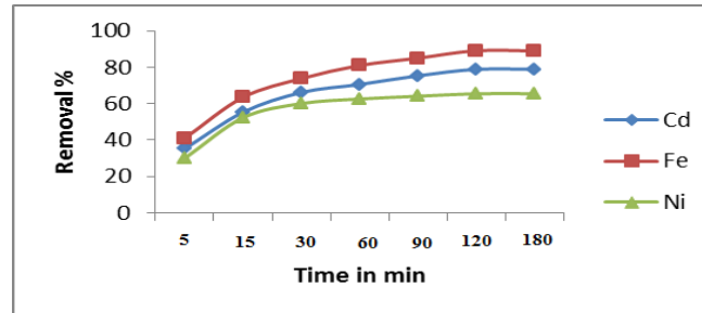
Figure 6. Contact time affecting on the removal of \text{Cd}^{+2} , \text{Fe}^{+3} and \text{Ni}^{+2} , from the solution ( C_i = 2 ppm, size < 0.5 mm, pH= 6, V=50\text{ml} , m=0.5\text{g} , t=180 min)
