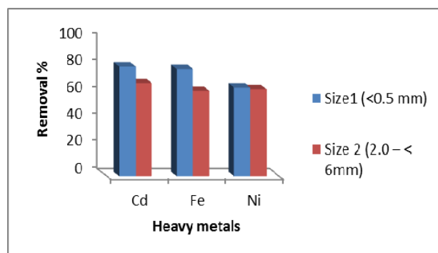
Figure 2. Adsorbent particle size affecting on the removal of Cd 2+ , Fe 3+ and Ni 2+ , from the solution (C i = 2 ppm · pH = 6 · m=0.5g · V=50ml · t=180 min)
