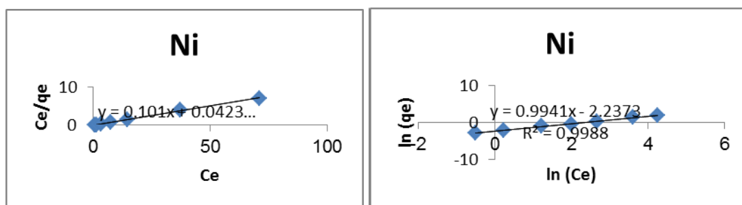
314 Figure 7. Adsorption isotherms of Cd +2 , Fe +3 and Ni +2 based on the Langmuir and 315 Freundlich models
