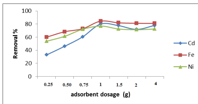
Figure 5. Adsorbent dose affecting on the removal of \text{Cd}^{+2} , \text{Fe}^{+3} and \text{Ni}^{+2} , from the solution ( C_i = 2 \text{ ppm} , size < 0.5 mm, pH= 6, V=50ml, t=180 min)
