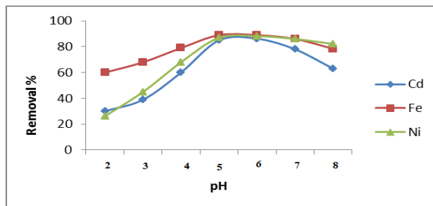
Figure 3. pH affecting on the removal of \text{Cd}^{+2} , \text{Fe}^{+3} and \text{Ni}^{+2} , from the solution ( C_i = 2 ppm, size < 0.5 mm, m=0.5\text{g} , V=50\text{ml} , t=180 min)
