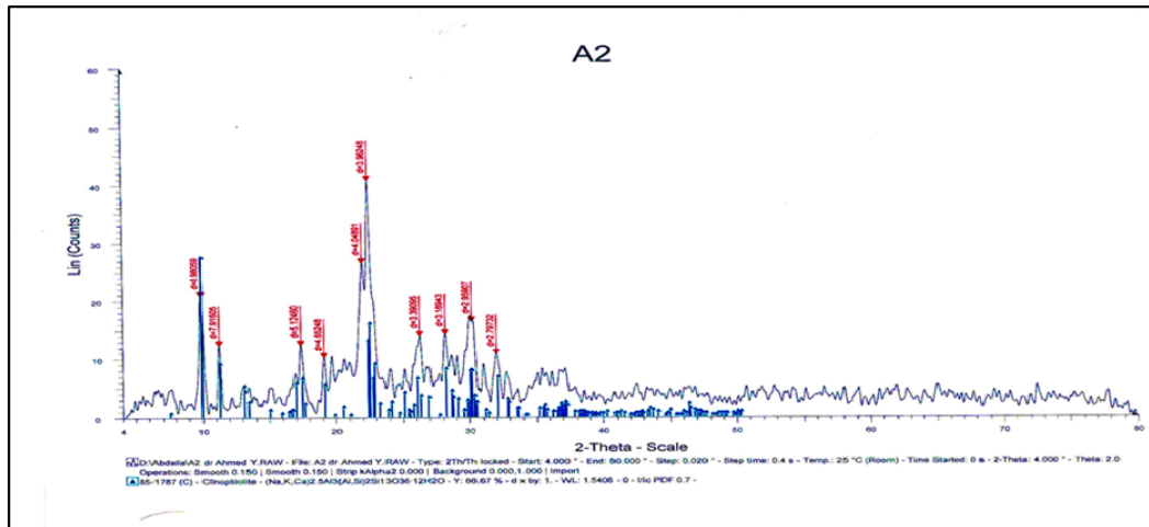
Figure 1. The XRD pattern of the sample confirming its Clinoptilolite mineralogy.
