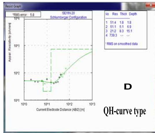
Fig 5: Geoelectric curve types
