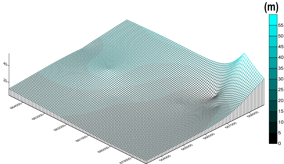
Fig 10: 3-D Wireframe map of weathered/fractured
