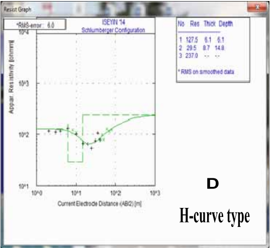
Fig 4: Geoelectric curve types
