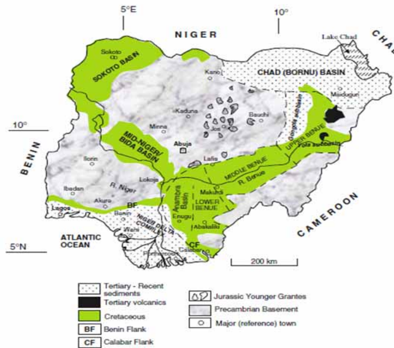
Fig 1: Geological map of Nigeria showing the basement complex and the sedimentary terrain. [11].
