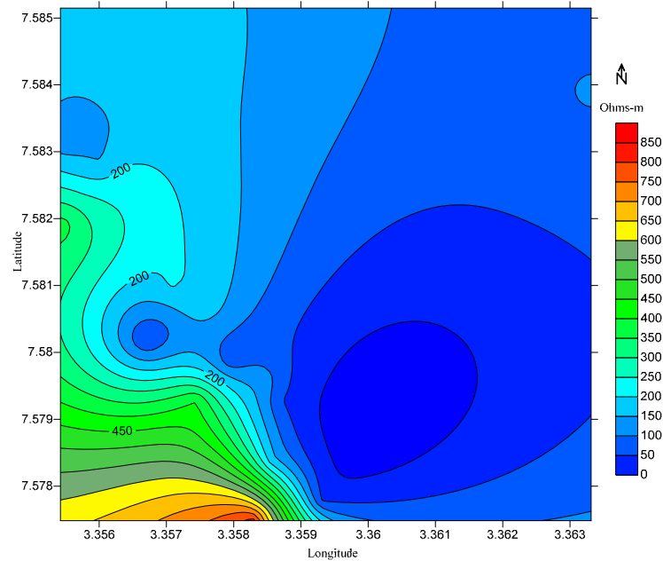
Fig 6: Isoresistivity map of topsoil
