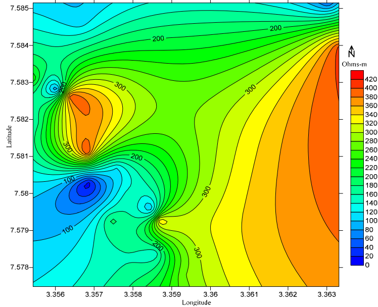
191 Fig 7: Isoresistivity of lateritic layer
