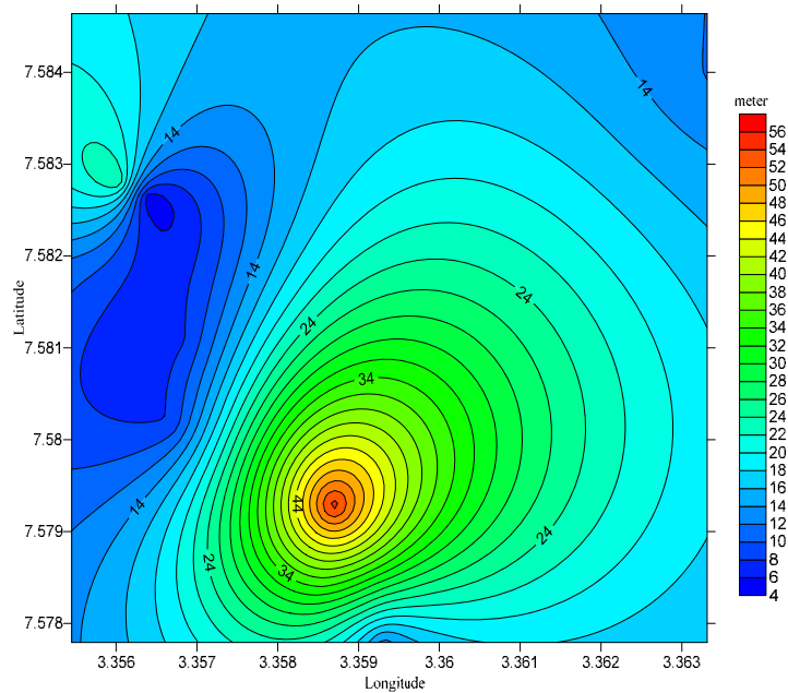
194 Fig 9: Isopach of weathered/fractured
