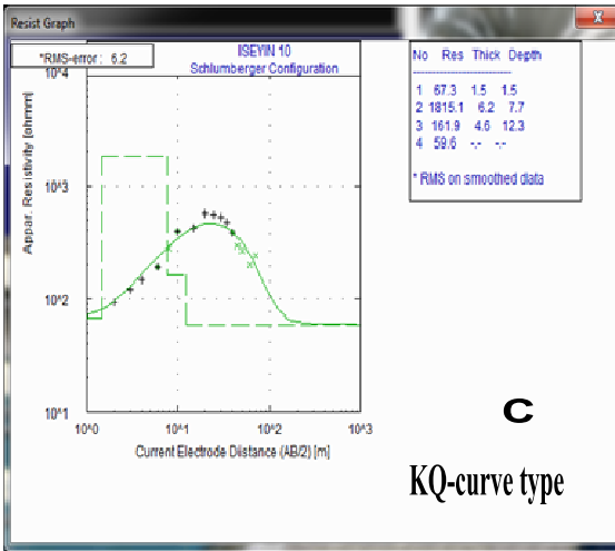
Fig 4: Geoelectric curve types
