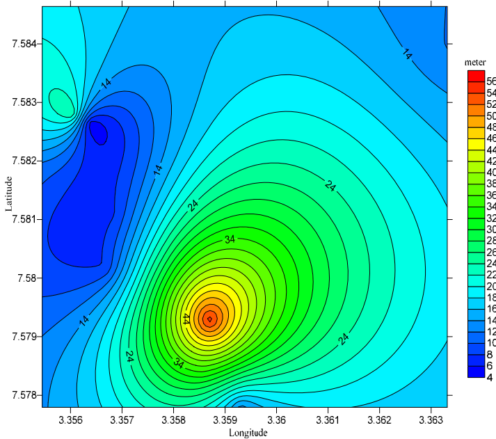
197 Fig 9: Isopach of weathered/fractured
