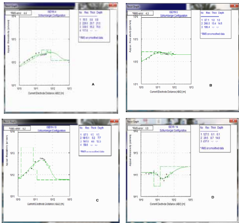
Fig 4: Geoelectric curve
