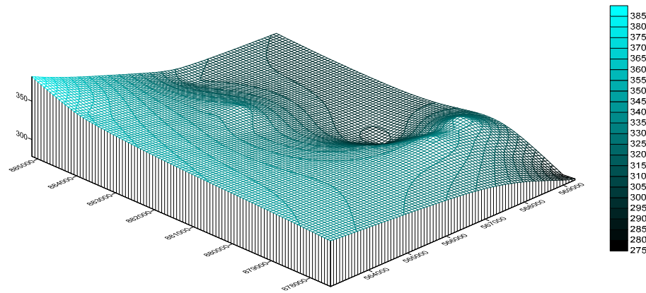
Fig 10: 3-D Wireframe map of weathered/fractured
