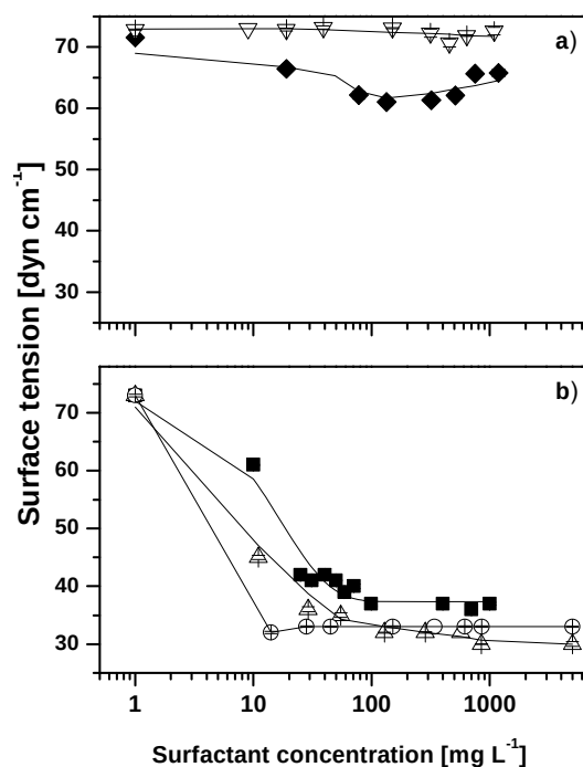
181 Figure 2. Surface tension as a function of nonionic surfactants concentration a) \blacklozenge 182 mesquite; \nabla guar gum. b) \blacksquare tween 80; \triangle canarcel 20; \circ eumulgin W-400. Bars mean 183 standard deviation with n=4 .
