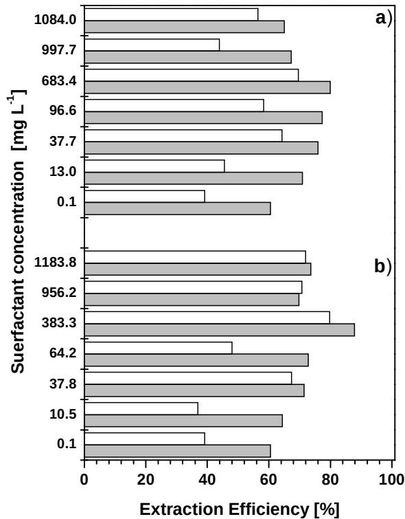
Figure 4. Extraction efficiency of ( \blacksquare ) \alpha -endosulfan and ( \square ) \beta -endosulfan with nonionic surfactants: a) guar gum; b) mesquite.
