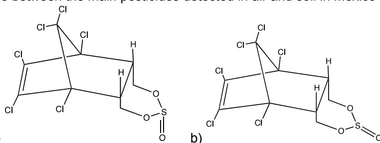
Figure 1. The molecular structure of a) \alpha -endosulfan and b) \beta -endosulfan.
