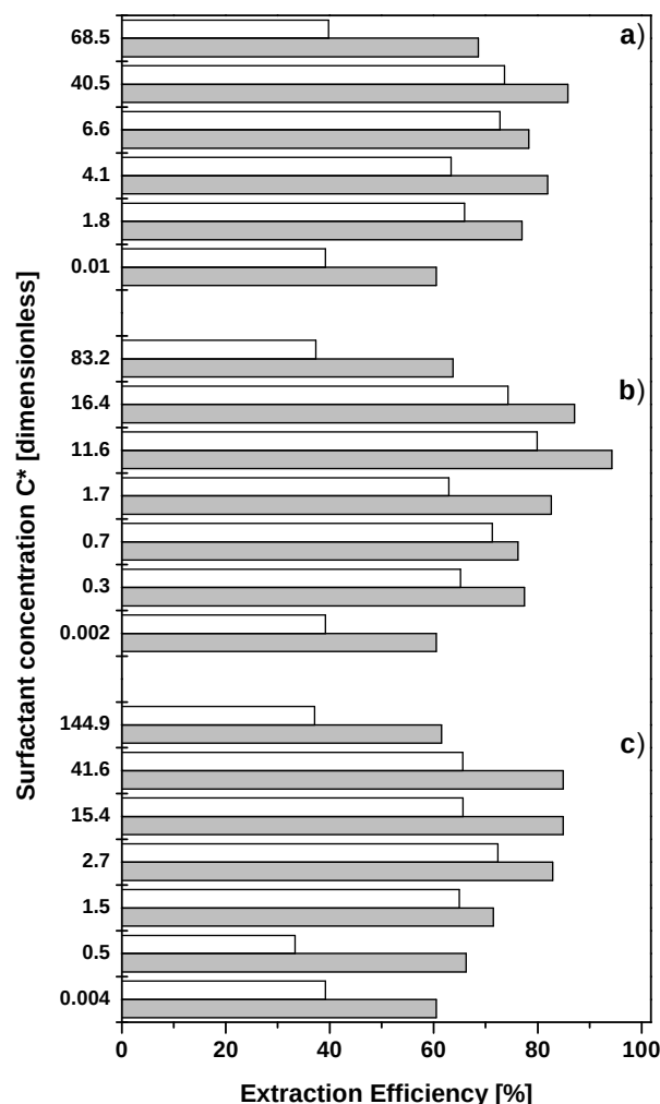
226 Figure 5. Extraction efficiency of (■) \alpha -endosulfan and (□) \beta -endosulfan with 227 nonionic surfactants a) tween 80; b) canarcel 20; c) eumulgin W-400. C^* = Surfactant 228 concentration/CMC. 229
