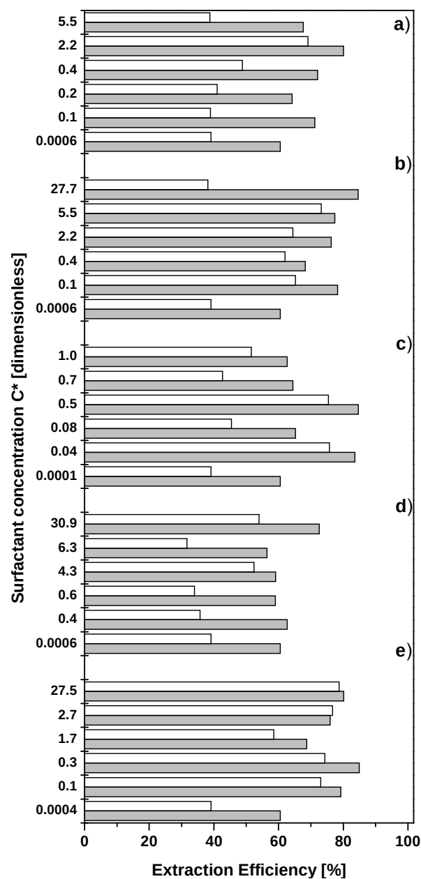
Figure 6. Extraction efficiency of ( \alpha -endosulfan and ( \beta -endosulfan with ionic surfactants a) dehyton KB; b) polafix LO; c) dehyquart; d) texapon KD; e) surfacpol A. C^* = Surfactant concentration/CMC.
