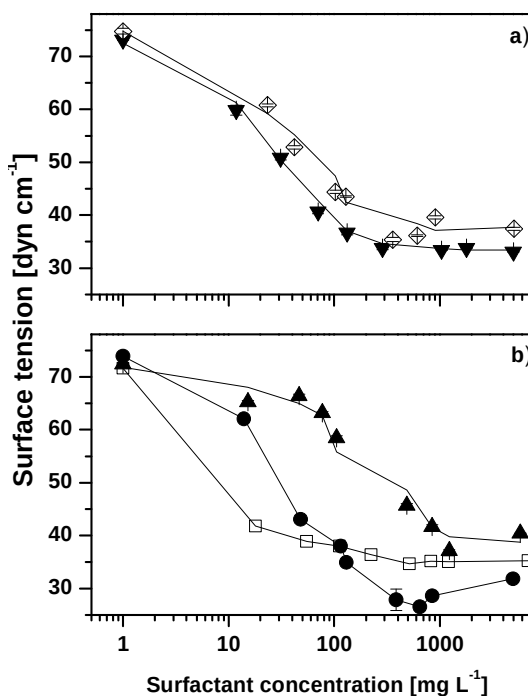
181 Figure 2. Surface tension as a function of nonionic surfactants concentration a) \blacklozenge 182 mesquite; \nabla guar gum. b) \blacksquare tween 80; \triangle canarcel 20; \circ eumulgin W-400. Bars mean 183 standard deviation with n=4 .
