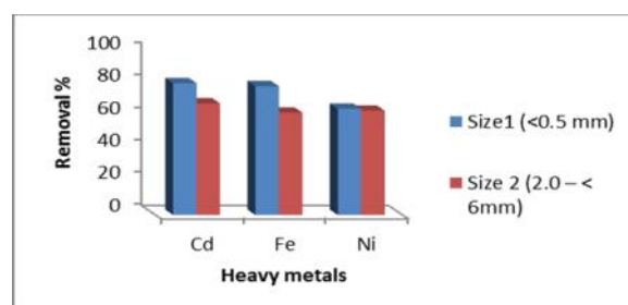
Fig 2. Adsorbent particle size affecting on the removal of Cd, Fe, and Ni, from the solution ( C_0=2 ppm · pH = 6 · m=0.5gr · V=50ml · T=180 min)
