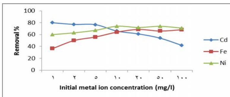
Fig. 4. Initial heavy metal ion concentration (mg/l) affecting on the removal of Cd, Fe, and Ni, from the solution (size < 0.5 mm, m=0.5gr, V=50ml pH = 6, T=180 min)
