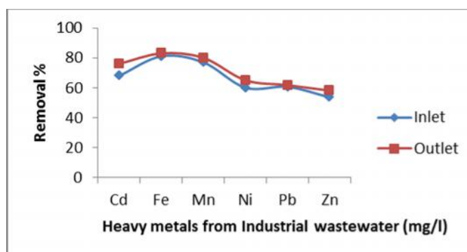
Fig. 8. Removal % of different heavy metals in both inlet and outlet samples from industrial wastewater after applying of zeolite.
