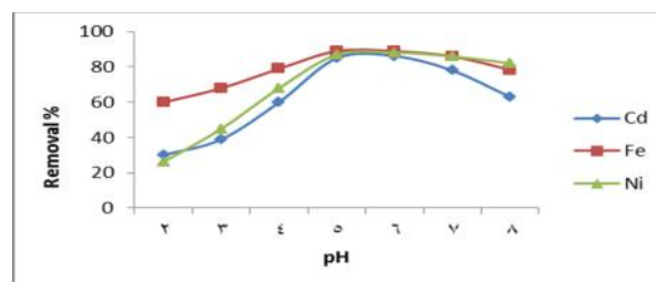
Fig. 3. pH affecting on the removal of Cd, Fe, and Ni, from the solution ( C_0=2 ppm · size < 0.5 mm · m=0.5gr · V=50ml · T=180 min)
