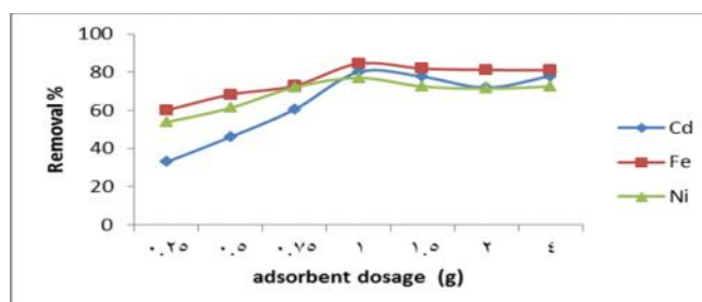
Fig. 5. Adsorbent dosage affecting on the removal of Cd, Fe, and Ni, from the solution (C 0 = 2 ppm, size < 0.5 mm, pH= 6, V=50ml, T=180 min)
