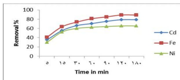
Fig. 6. Contact time affecting on the removal of Cd, Fe, and Ni, from the solution ( C_0=2 ppm, size < 0.5 mm, pH= 6, V=50ml, T=180 min)
