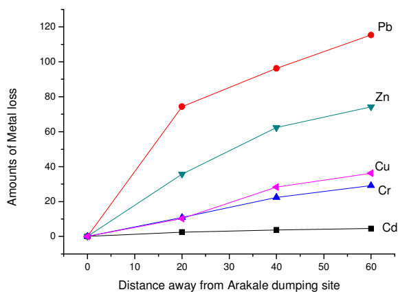
Figure 2: Amounts of metal loss when moving away from Arakale dumping site
