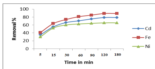
Figure 6. Contact time affecting on the removal of \text{Cd}^{+2} , \text{Fe}^{+3} and \text{Ni}^{+2} , from the solution ( C_i = 2 \text{ ppm} ; size < 0.5 \text{ mm} ; pH= 6; V=50ml; m=0.5g)
