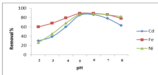
Figure 3. pH affecting on the removal of \text{Cd}^{+2} , \text{Fe}^{+3} and \text{Ni}^{+2} from the solution ( C_i = 2 \text{ ppm} ; size < 0.5 \text{ mm} ; m = 0.5\text{g} ; V = 50\text{ml} ; t = 180 \text{ min} )
