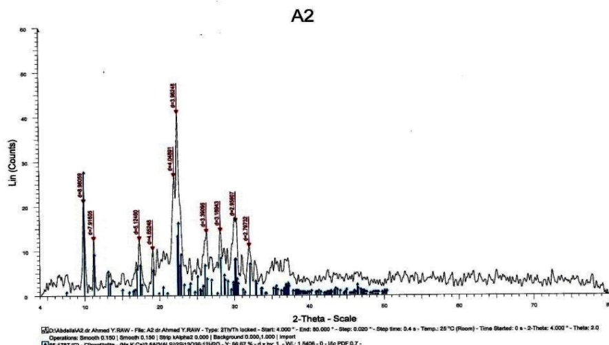
Figure 1. The XRD pattern of the sample confirming its Clinoptilolite mineralogy.
