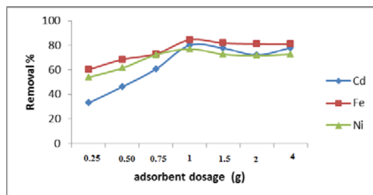
Figure 5. Adsorbent dose affecting on the removal of \text{Cd}^{+2} , \text{Fe}^{+3} and \text{Ni}^{+2} , from the solution ( C_i = 2 ppm; size < 0.5 mm; pH= 6; V=50ml; t=180 min)
