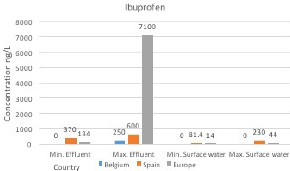
Figure 8b: Occurrence and concentration of ibuprofen in effluent and surface water around world 2006-2013
