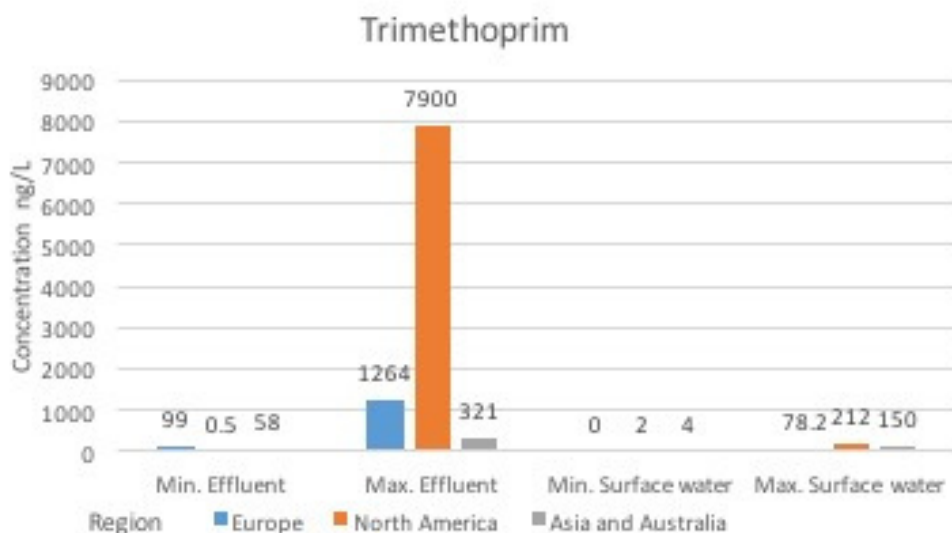
Figure 2 a: Occurrence and concentration of trimethoprim in effluent and surface water around world 2006-2013
