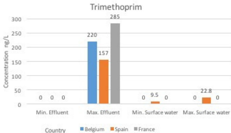
Figure 2 b: Occurrence and concentration of trimethoprim in effluent and surface water around Europe 2006-2013
