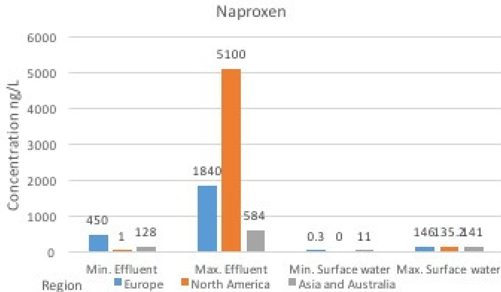
Figure 9: Occurrence and concentration of naproxen in effluent and surface water around world 2006-2013
