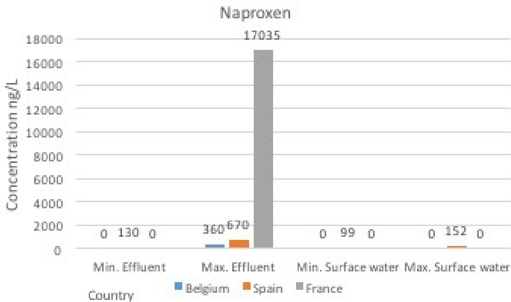
Figure 9: Occurrence and concentration of naproxen in effluent and surface water around world 2006-2013
