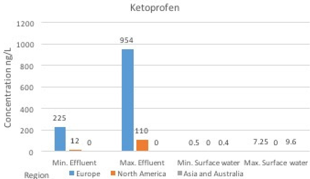
Figure 7a: Occurrence and concentration of Ketoprofen in effluent and surface water around world 2006-2013
