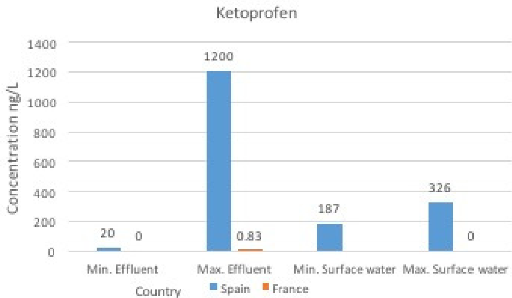
Figure 7b: Occurrence and concentration of Ketoprofen in effluent and surface water around Europe 2006-2013
