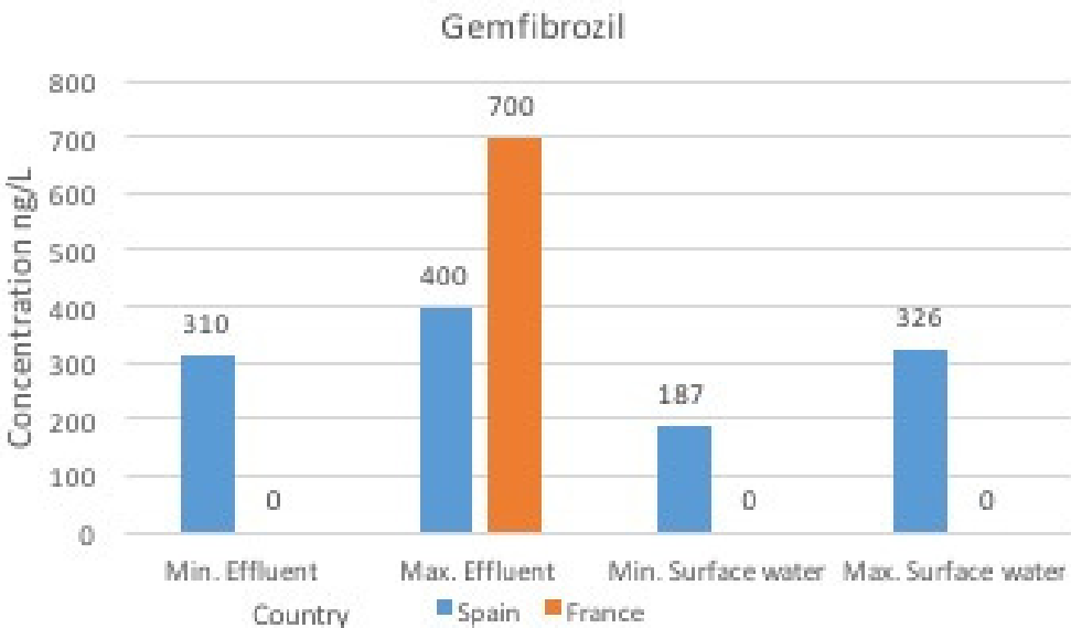
Figure 6b: Occurrence and concentration of Gemfibrozil in effluent and surface water around Europe 2006-2013
