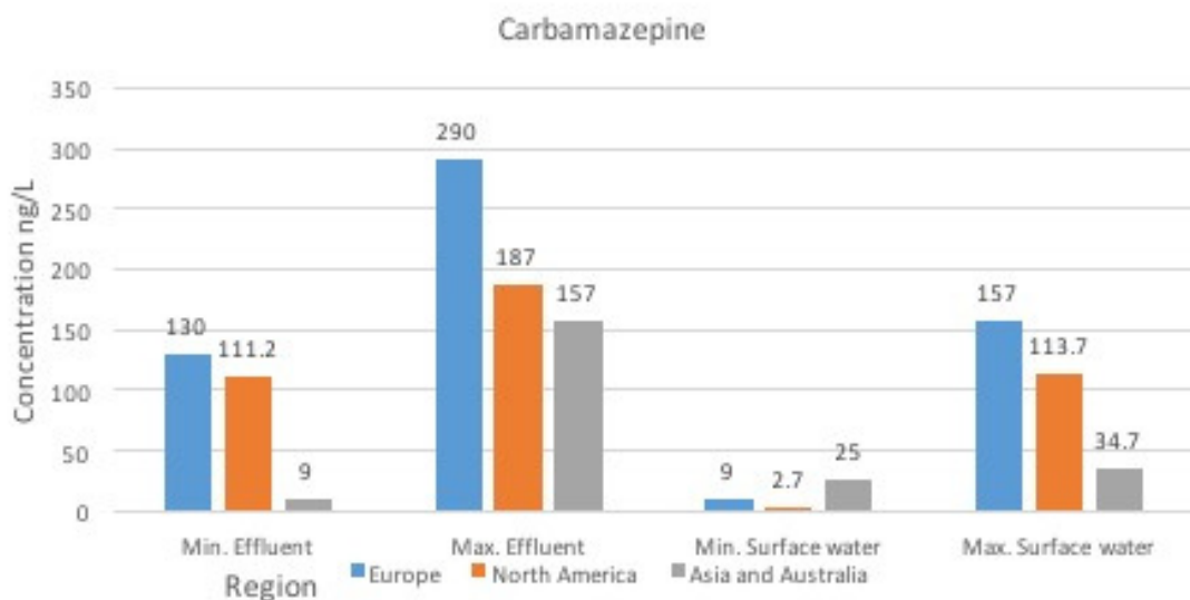
Figure 1a: Occurrence and concentration of carbamazepine in effluent and surface water around world 2006-2013
