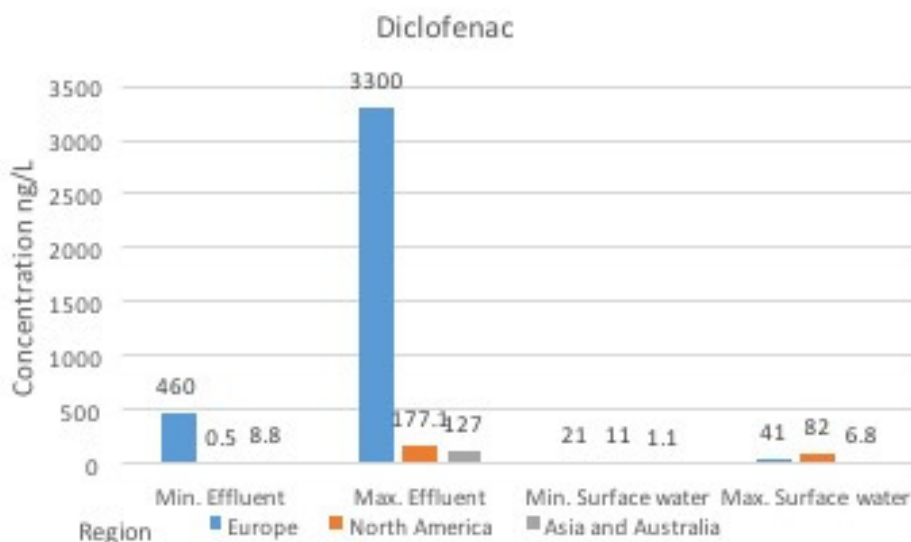
Figure 3a Occurrence and concentration of diclofenac in effluent and surface water around world 2006-2013
