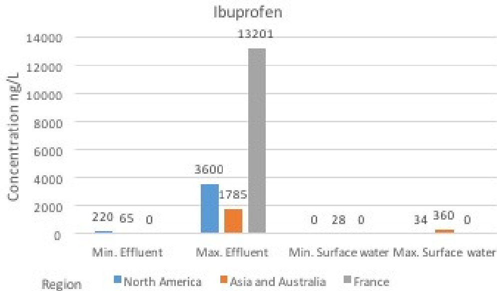
Figure 8a: Occurrence and concentration of ibuprofen in effluent and surface water around world 2006-2013
