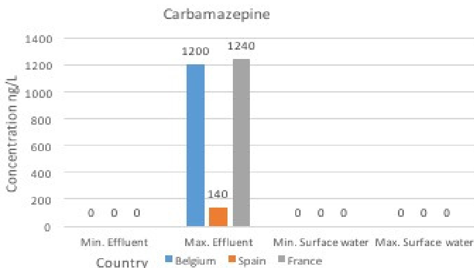
Figure 2b: Occurrence and concentration of carbamazepine in effluent and surface water around Europe 2006-2013
