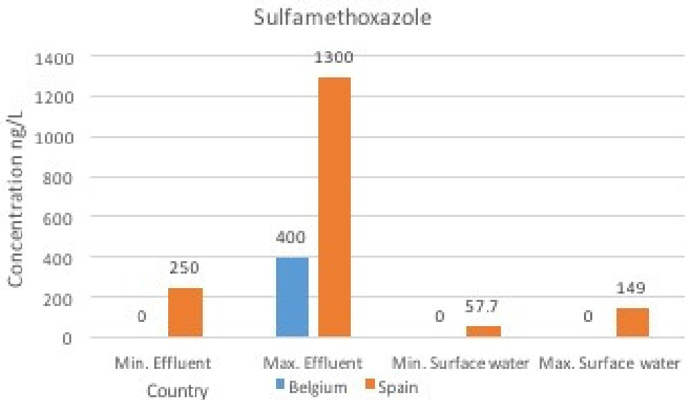
Figure 5b: Occurrence and concentration of sulfamethoxazole in effluent and surface water around Europe 2006-2013
