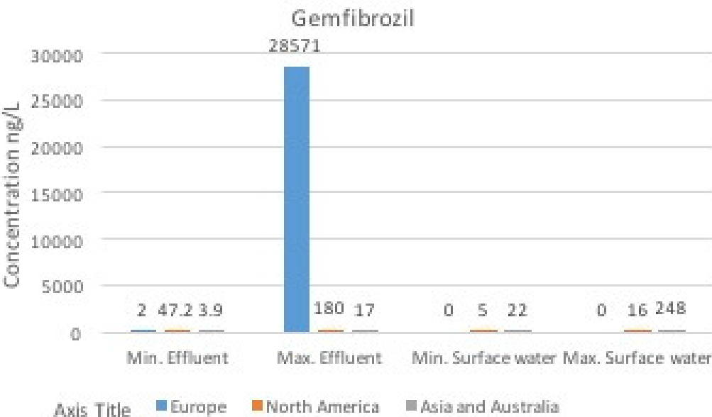
Figure 6a: Occurrence and concentration of gemfibrozil in effluent and surface water around world 2006-2013
