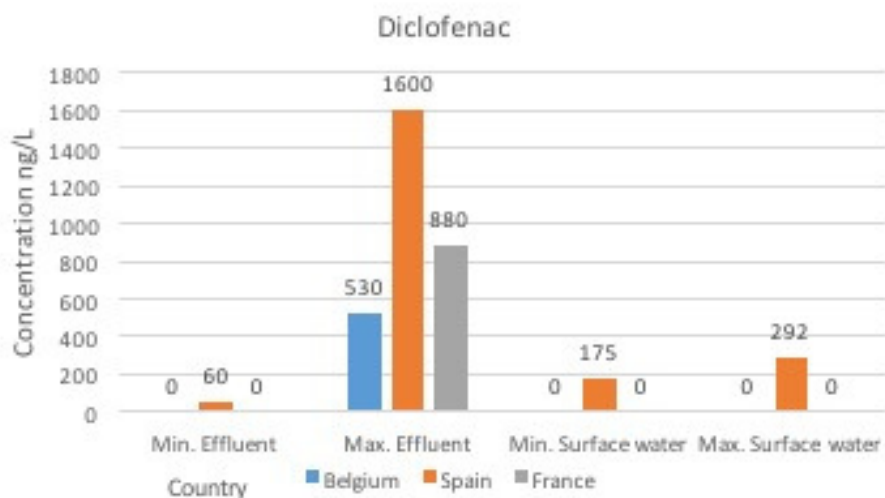
Figure 3b Occurrence and concentration of diclofenac in effluent and surface water around Europe 2006-2013
