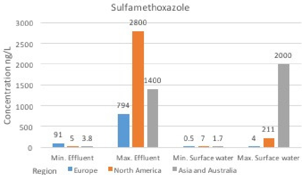
Figure 5a: Occurrence and concentration of sulfamethoxazole in effluent and surface water around world 2006-2013
