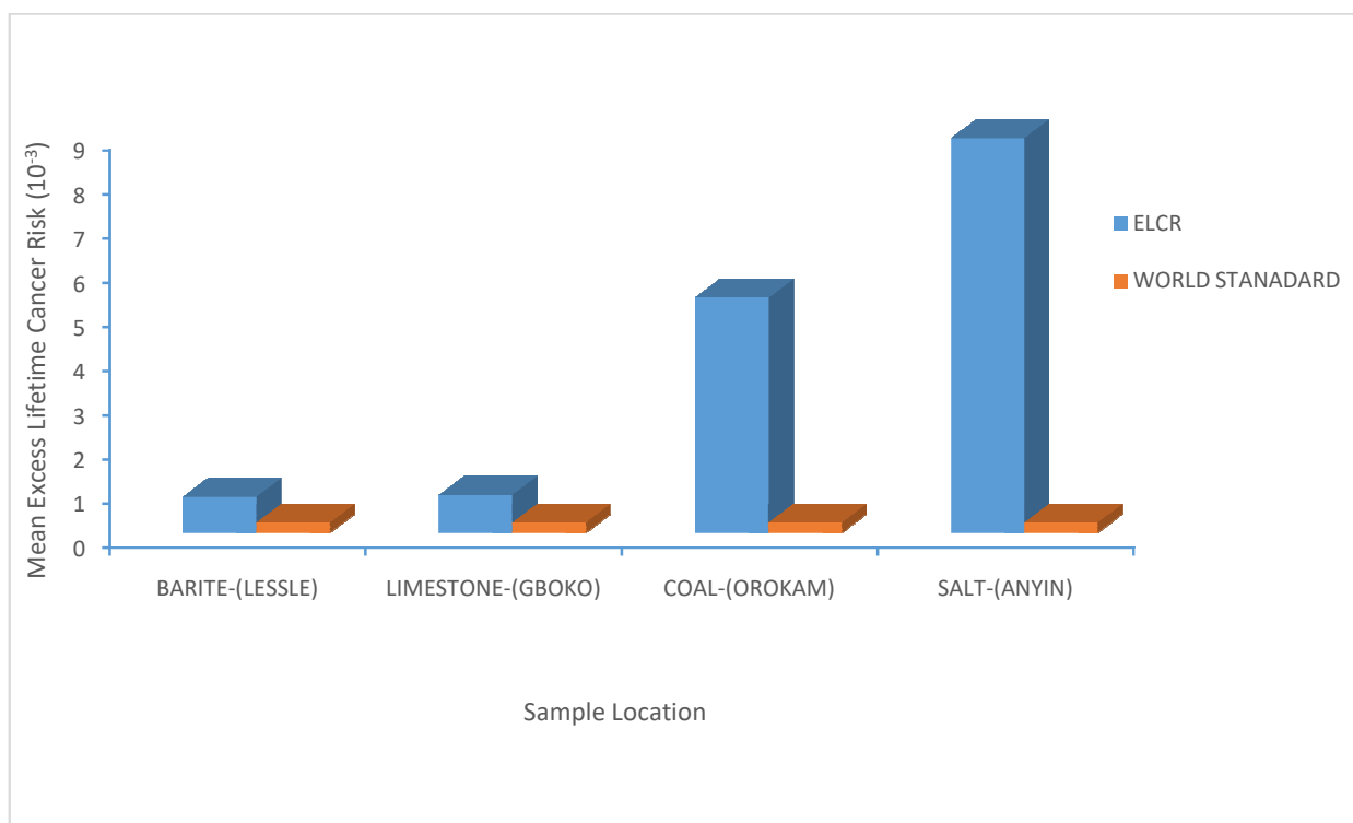
Fig. 3: Comparison of Mean ELCR of mineral deposition field with World Safe Limit Value
