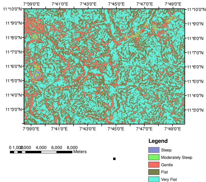
Figure 3: Slope map within the Study area.
