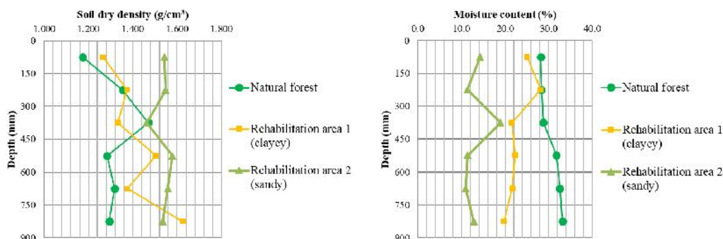
Fig. 6. Results of soil dry density and moisture content
