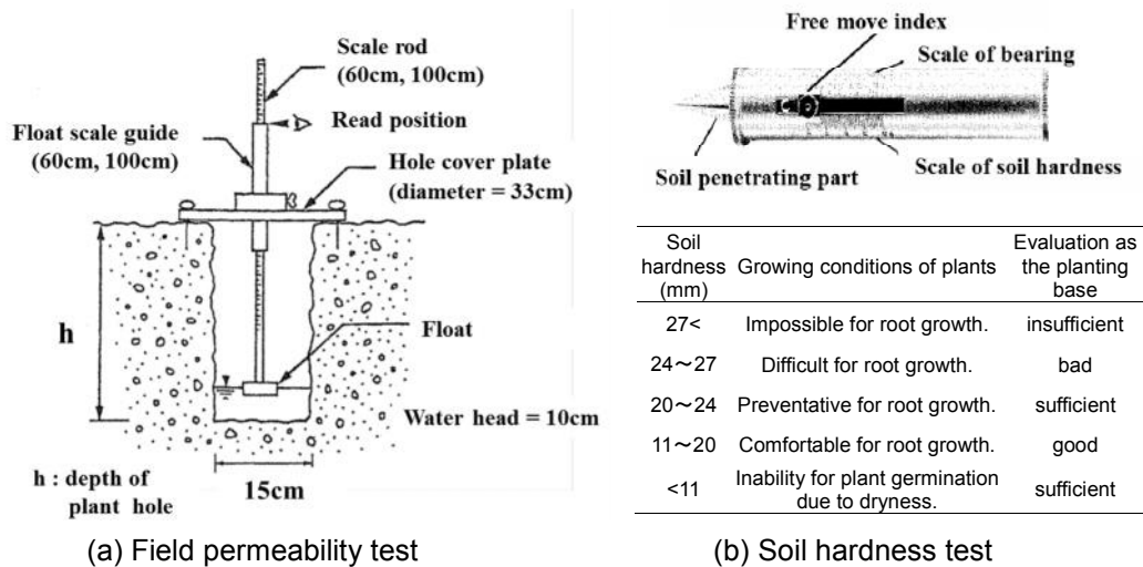
Fig. 4. Field research equipment
