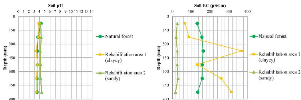
Fig. 7. Results of soil pH and EC
