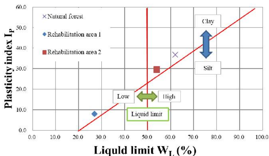
Fig. 5. Plasticity chart
