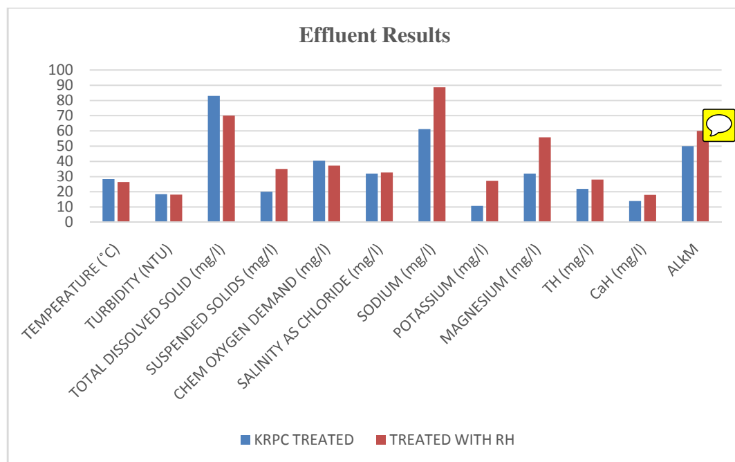
Figure 2: Temperature, Turbidity, and Concentration of Solids, Anions and Metals in KRPC and RH treated Effluents
