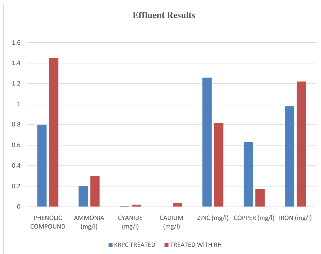
Figure 4: Concentration of Different Compounds in KRPC and RH treated Effluents
