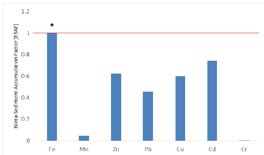
Figure 3- Biota-Sediment Accumulation factors (BSAF) of trace metals in M. vollenhovenii NOTE: BAF values of 1 and above signify significant values; indicated by the red line. Asterisk bars indicate trace metals of significant BAF.
