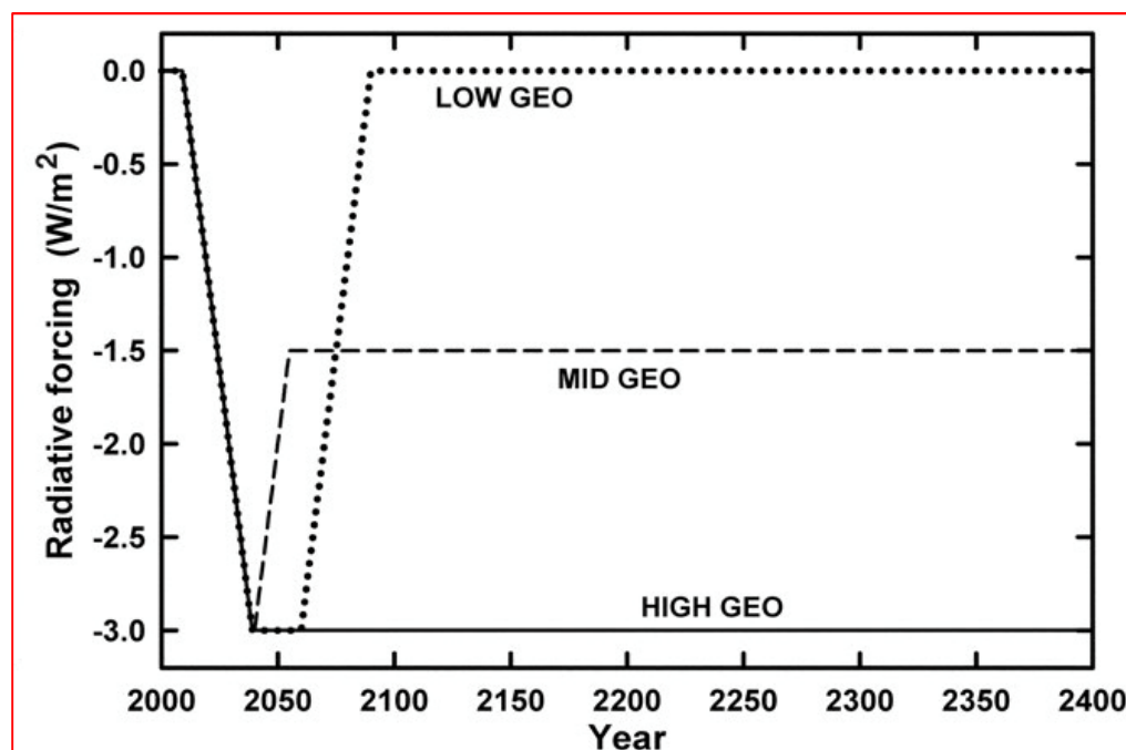
248 Fig 3. Reduction of incoming solar radiative forcing based on different geoengineering scenarios. LOW GEO indicates no direct 249 human intervention on modification of climate. HIGH GEO indicates scenario of which released of H 2 S and SO 2 through aerosol 250 injection are similar to eruption of Mount Pinatubo for every 2 years. MID GEO indicates mid-level intervention by human whereby 251 aerosol injections are introduced over longer interval period of time. (4)
