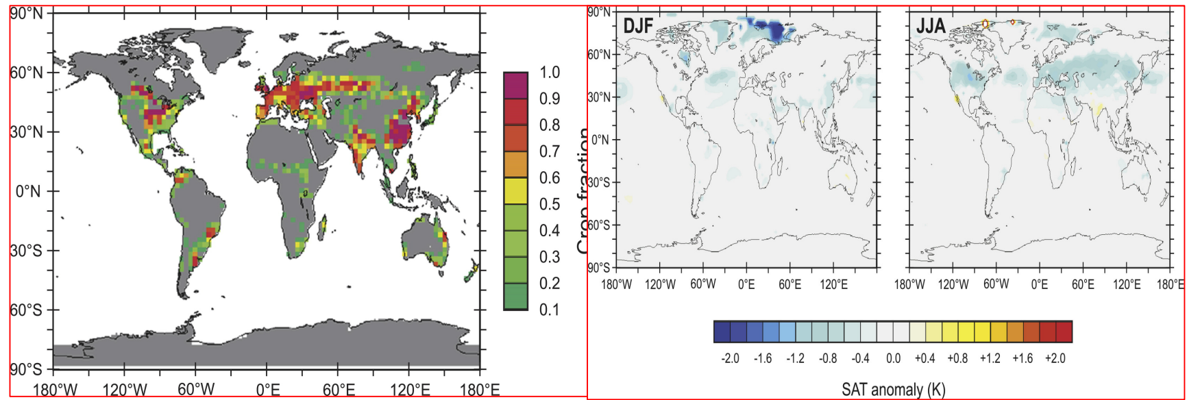
Fig 2. Global crop distribution and cooling associated with albedo-engineered crops. (Left) Diagram illustrates Earth’s surfaces model if covered by albedo-engineered agriculture crops. (Right) Diagram illustrates temperature anomaly taken during December-January-February (DJF) and June-July-August (JJA) if global agriculture surface are covered with albedo-engineered crops. Note that patches above the Northern Hemisphere are corresponding to sea-ice feedback during winter and summer solstices. (17)
