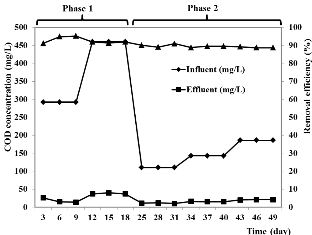
185 Fig. 2. Chemical oxygen demand removal efficiency of constructed wetland model 186 during time course.
