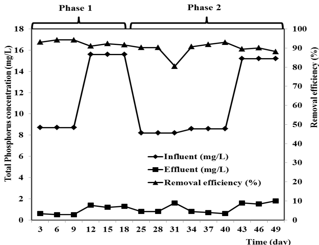
Fig. 5. Total phosphorus removal efficiency of constructed wetland model during time course.
