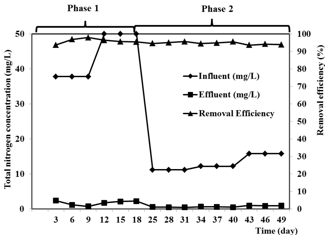
210 Fig. 3. Total nitrogen removal efficiency of constructed wetland model during time 211 course.
