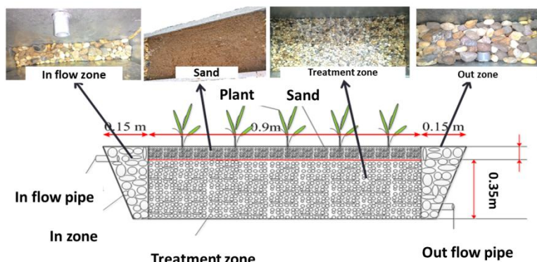
Fig. 1. Schematic of constructed wetland system
