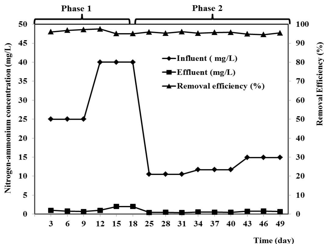
231 Fig. 4. Nitrogen-ammonium removal efficiency of constructed wetland model during 232 time.
