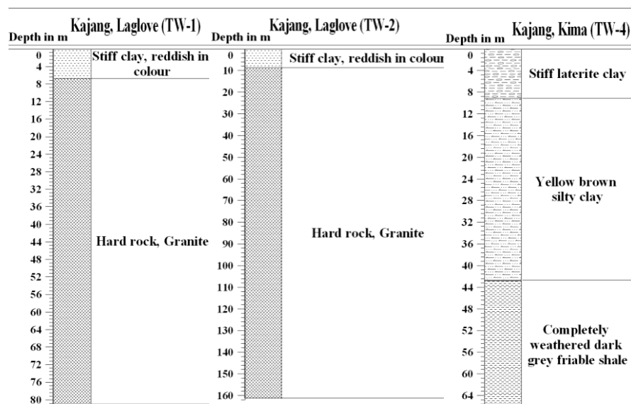
Fig.3. Subsurface well logs of Kajang Town.
