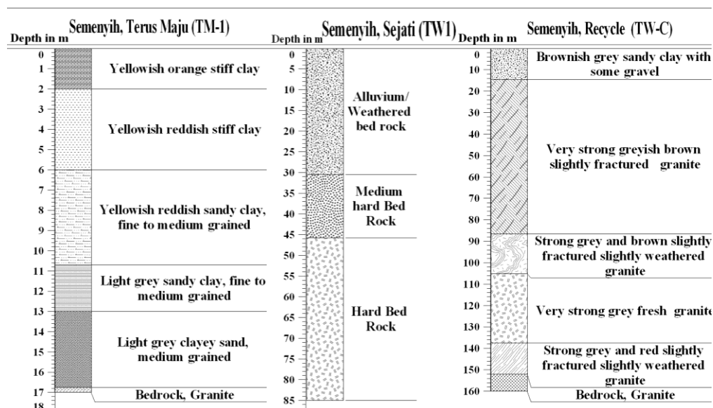
Fig. 4. Subsurface well logs of Semenyih Town.
