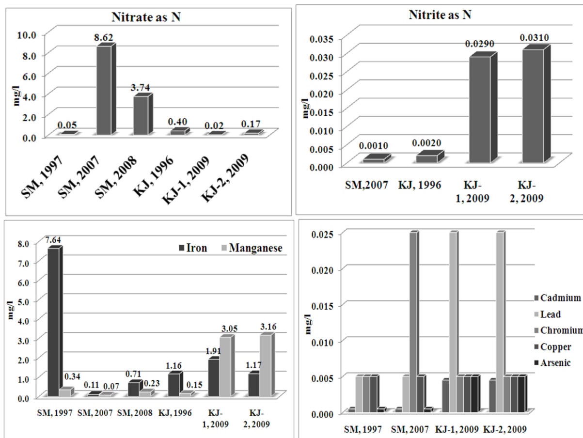
Fig. 6. Nitrate, nitrite, iron, manganese and trace element concentrations of the wells.
