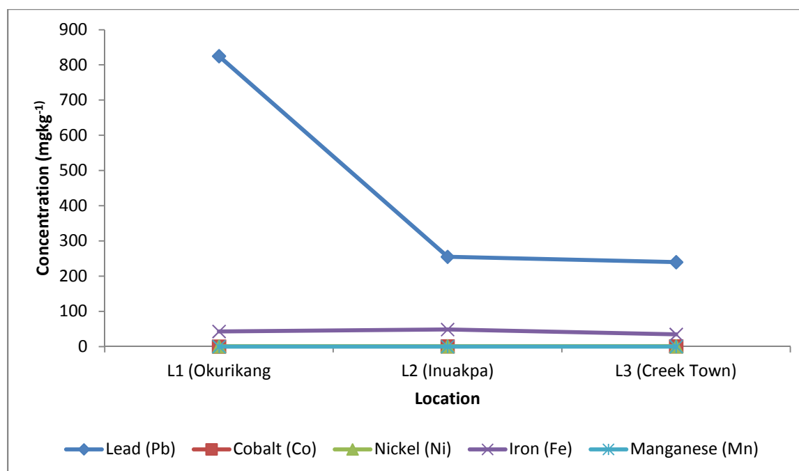
FIGURE 2: Mean concentrations and distribution of heavy metals in the three sampling locations.
