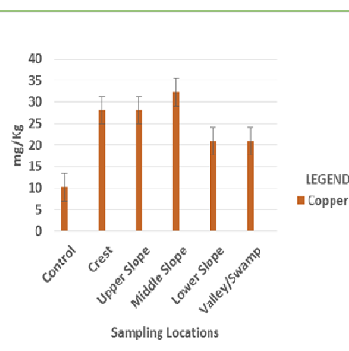
FIG. 9: Concentration of Copper in the municipal dump site in Calabar
