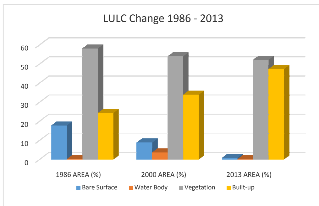
Figure 6: LULC change 1986 - 2013
