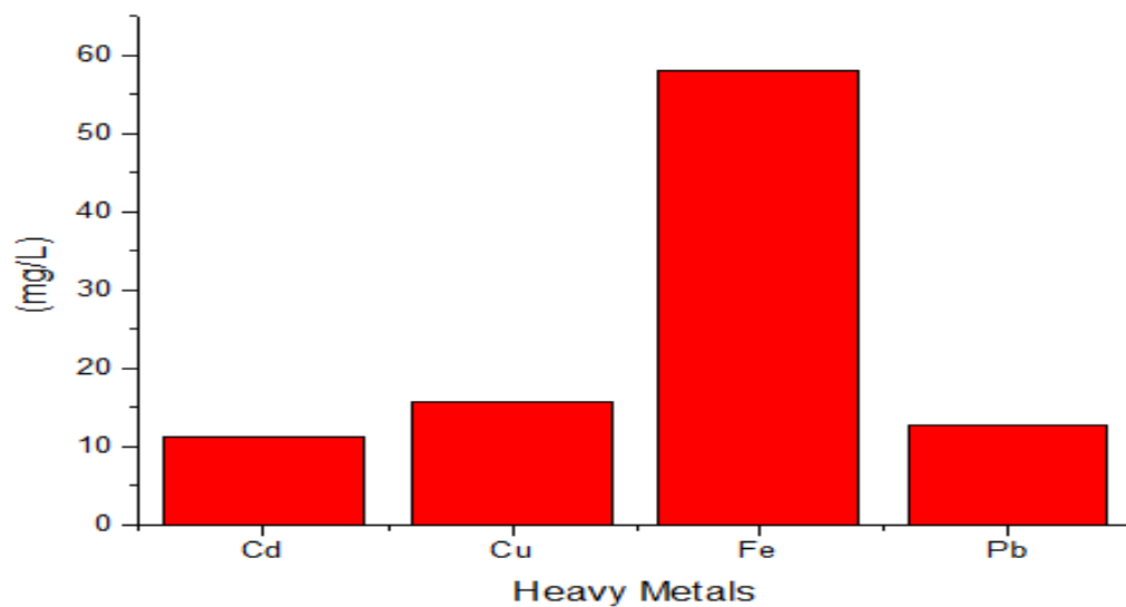
262 Figure 5: Heavy metal concentration levels at the near the waste dumpsite.
