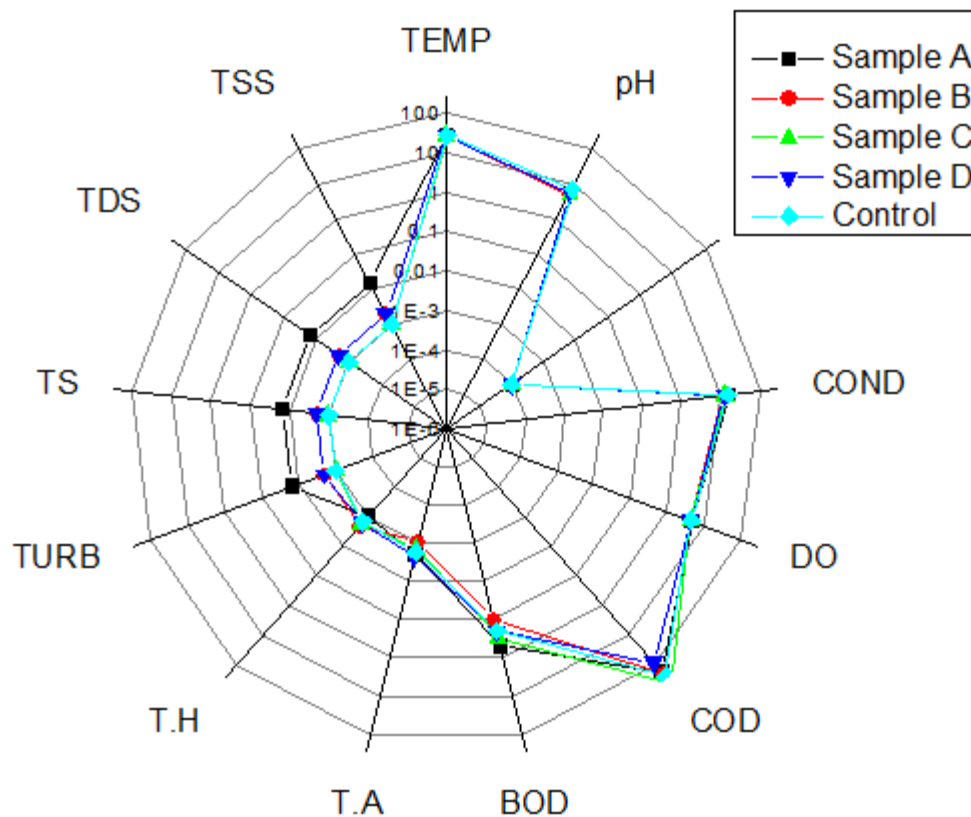
Figure 3: Radial plot showing the physio-chemical values of water samples in Nekede Mechanic village.
