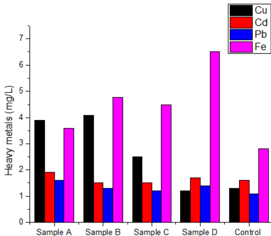
Figure 4: concentration of heavy metals in the soil samples.
