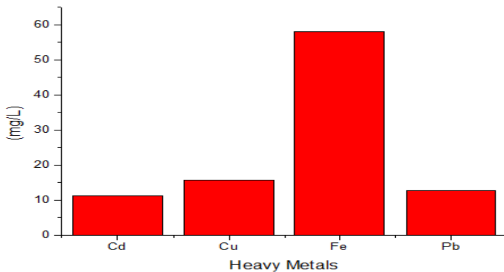
259 Figure 5: Heavy metal concentration levels at the near the waste dumpsite.
