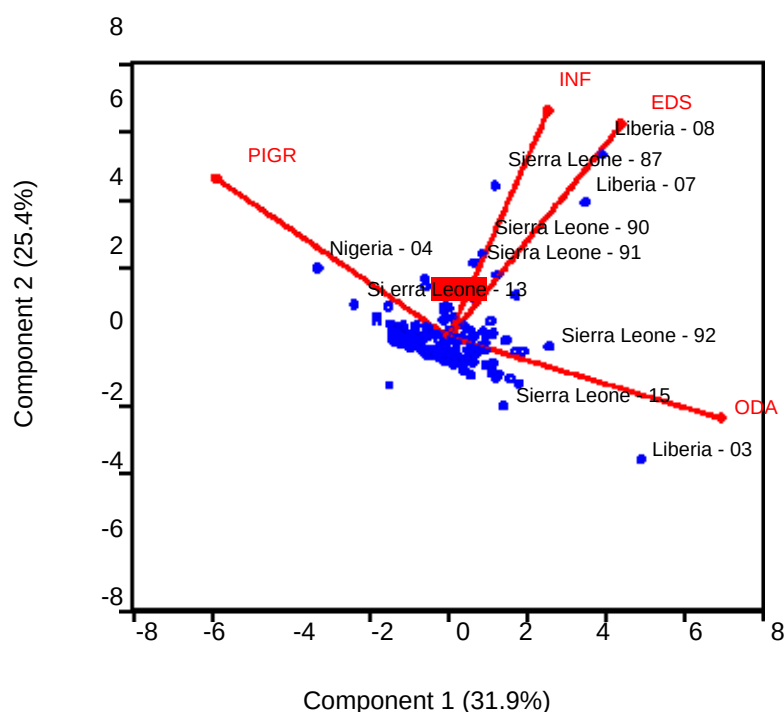
Figure 2. Orthonormal Loading Output
