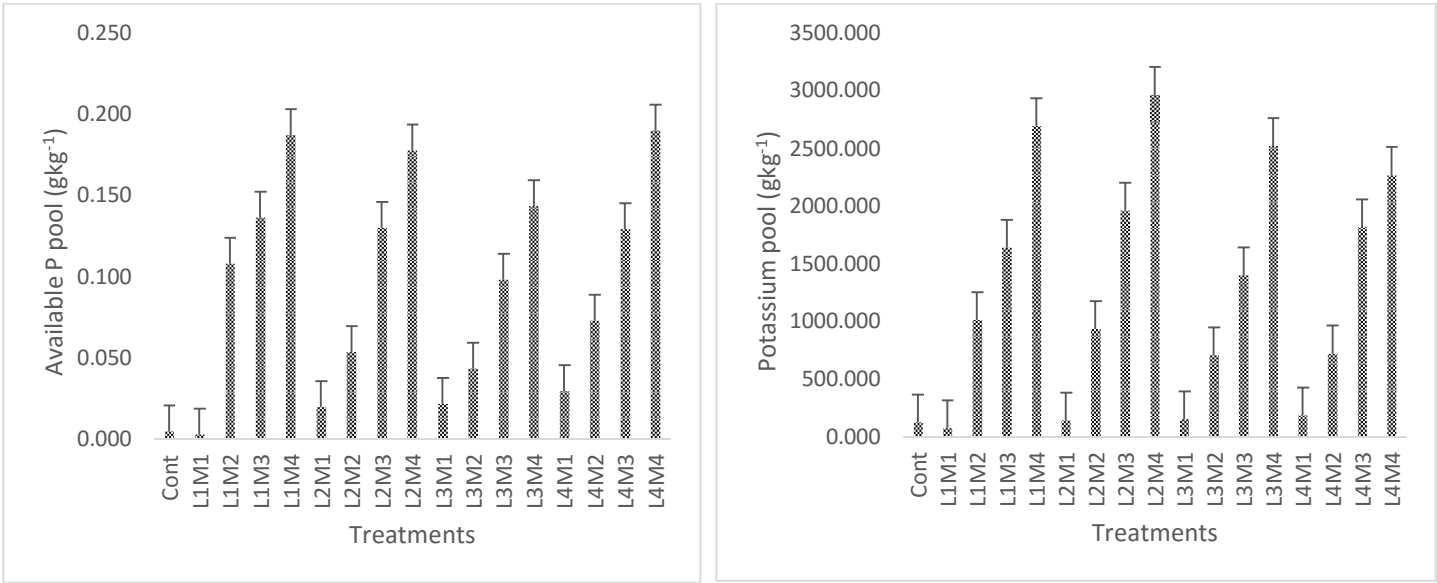
Fig. 1a Effects of Moringa Seed Powder and Liquid Gold on soil P Fig. 1b Effects of Moringa Seed Powder and Liquid Gold on soil K
