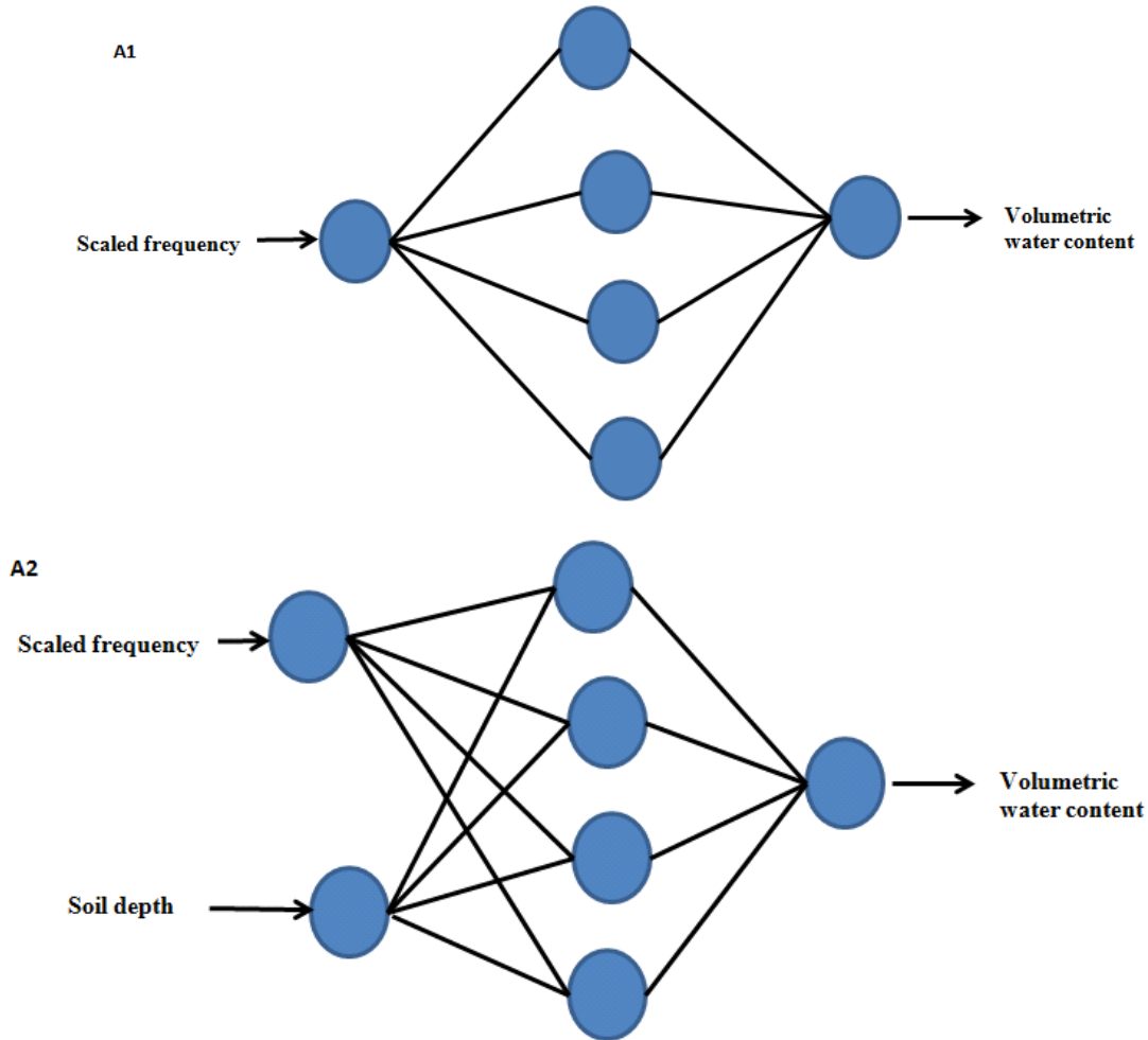
175 Fig. 2. Structure of the best ANN used in this study in the case of one inputs (A1) and in the case of 176 two inputs (A2). 177 178 179
