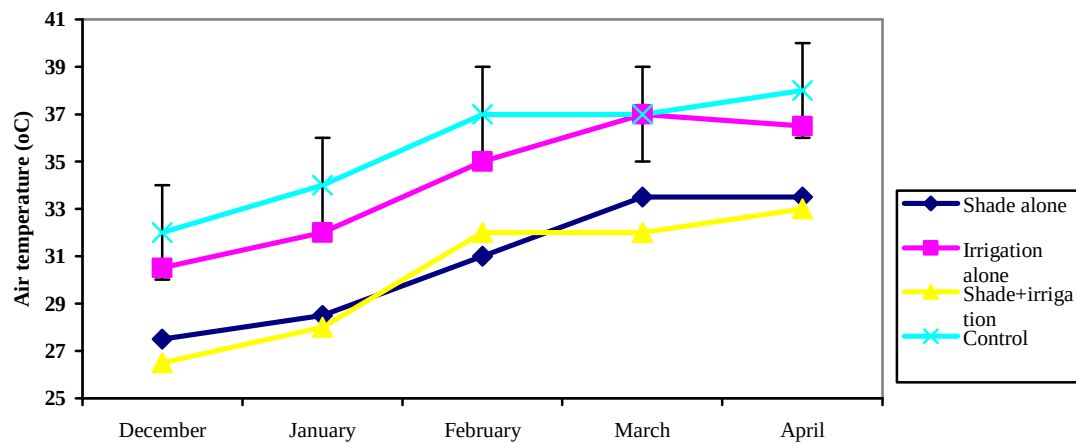
Figure 2: Effects of shade and irrigation on air temperature variation within cacao canopy
