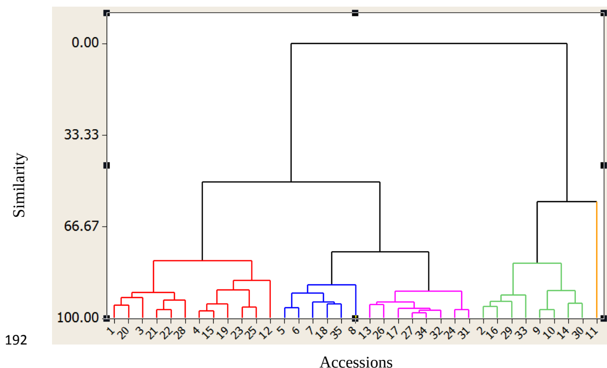
193 Fig. 1. The dendrogram of 9 morphological traits derived from 35 Jatropha curcas accessions
